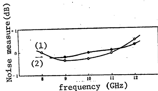
(a) No 1 amplifier (TRW0.5um FET)
