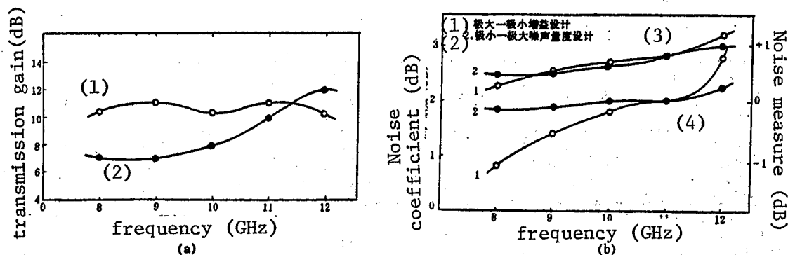
Fig. 8 Transmission gain, noise coefficients, and noise measures of No 1 amplifier
