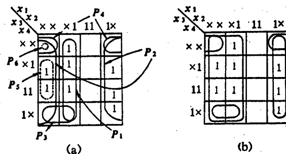
Fig. 4 Two Covering Selections
