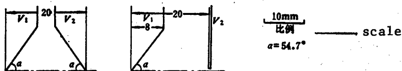
(a) hyperboloid field dual potential (b) Munro simplified type
