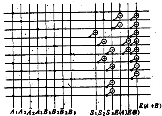
Fig. 2 Tri-bit Half-adder
