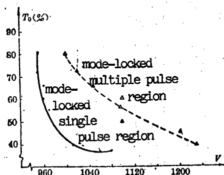
Fig. 4. Dye concentration versus mode-locking threshold
