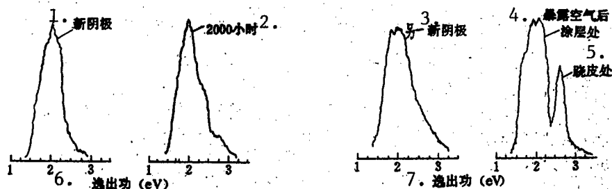
Figure 3. Distribution of Ternary Salt Work Function Measured with a Low Energy Scanning Electron Probe
