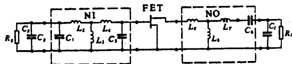
Fig. 7 No 1 Amplifier Wiring Diagram
