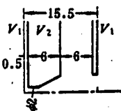
(a) hyperboloid field dual potential (b) Munro simplified type
