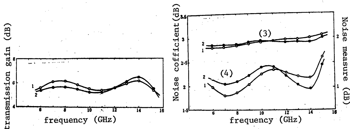
Fig. 10 Transmission Gain, Noise Coefficients, and Noise Measure of No 2 Amplifier
