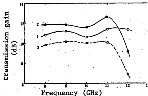
Fig. 1 FET Non-unilateral Characteristics and the Effect of Network Loss on the Amplifier Gain (TRW 0.5 \mu m FET)
