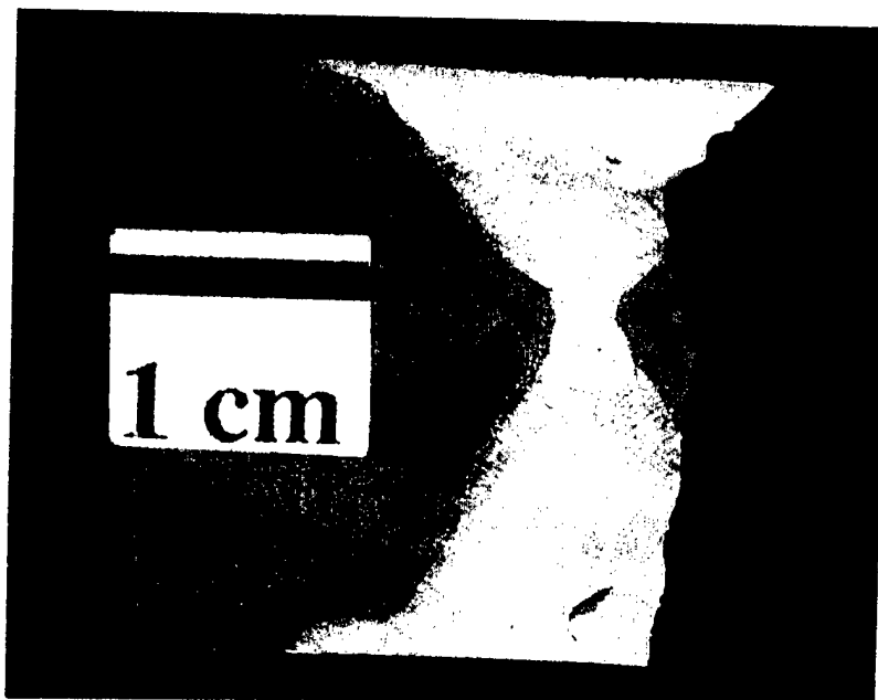
Figure 6.3.4: Macrograph of cross-section (from TM-5) at location that exposes the initial flaw at the convex side of the fracture face. (Top side is the convex surface).
