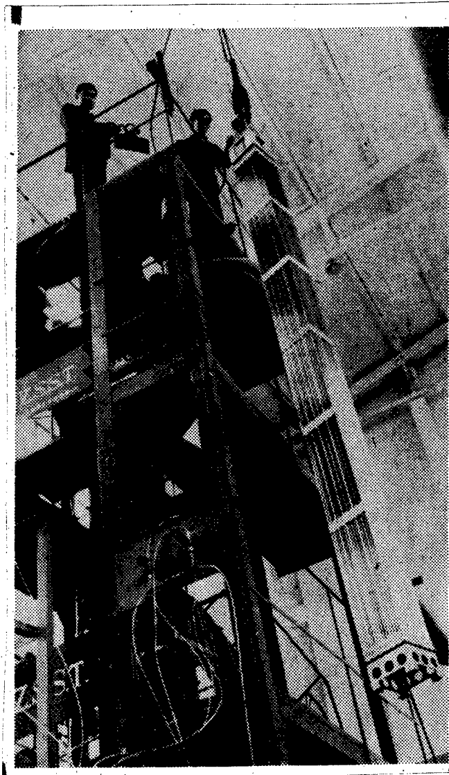
Personnel working on nuclear power plant's construction conducting water blockage tests on nuclear fuel elements.
