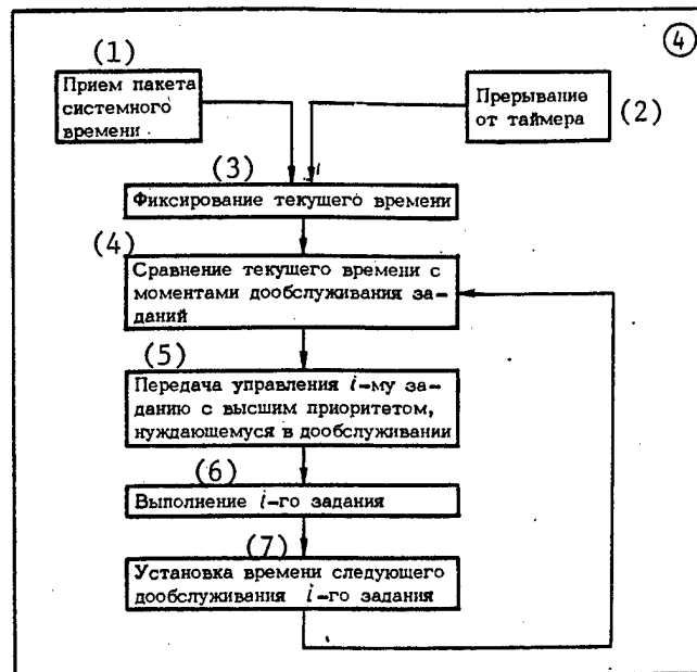
Figure 4. Block Diagram of Algorithm for Real-Time Fulfillment of Tasks
