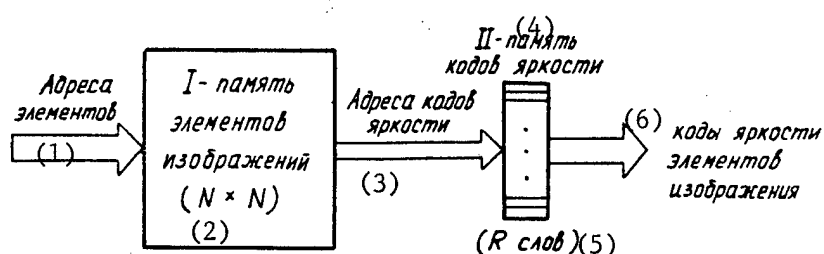
Fig. 9. Structure of memory block with indirect addressing
