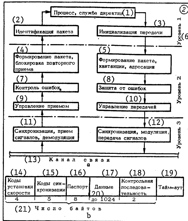
Figure 2. Structure of Exchange Protocol (a) and Format of Data Packet (b)
