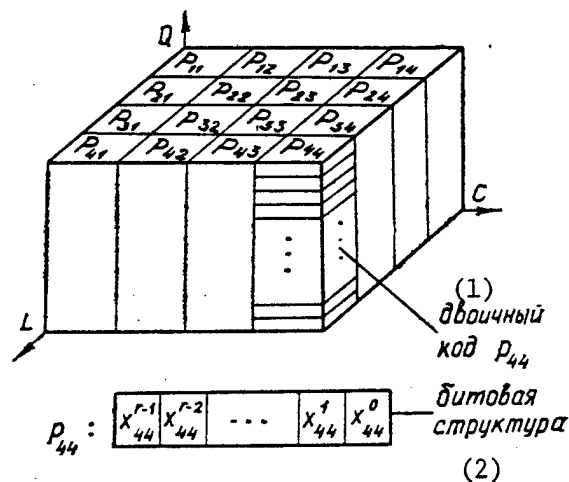
Fig. 6. Bit structure of array of data p_{ij}
