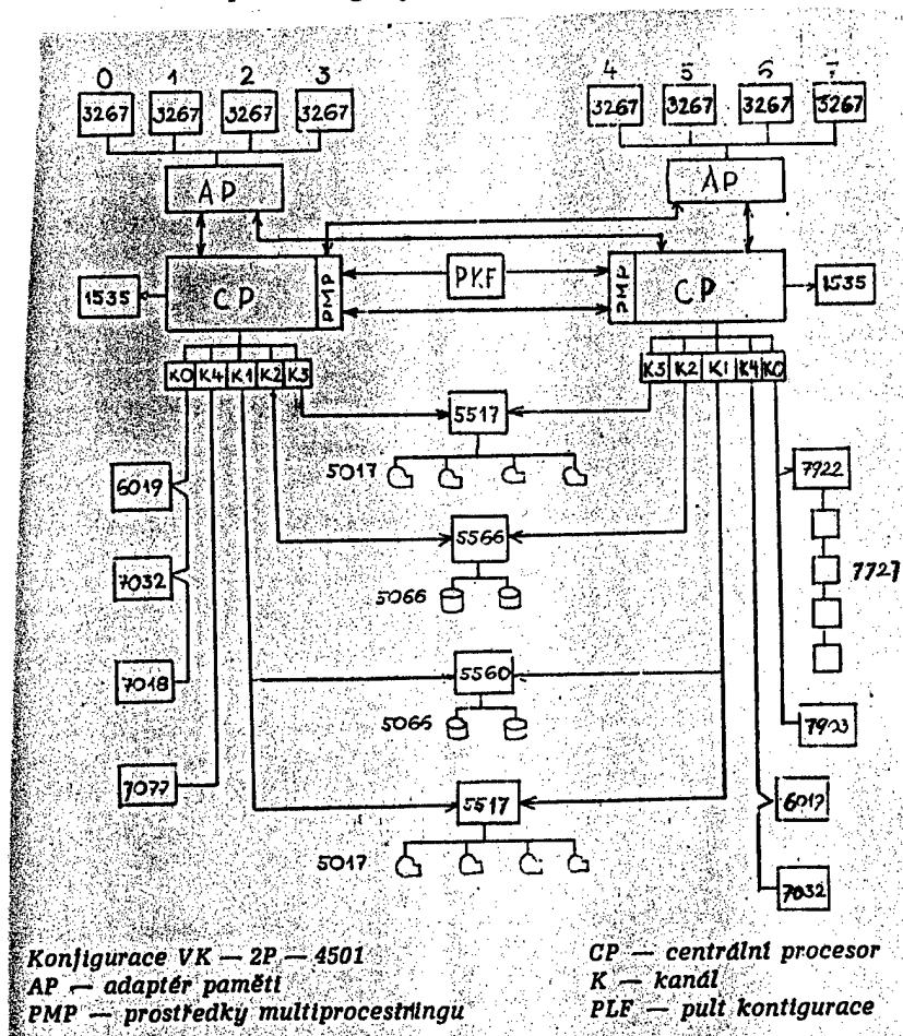
Configuration of VK-2P-45.01 System
