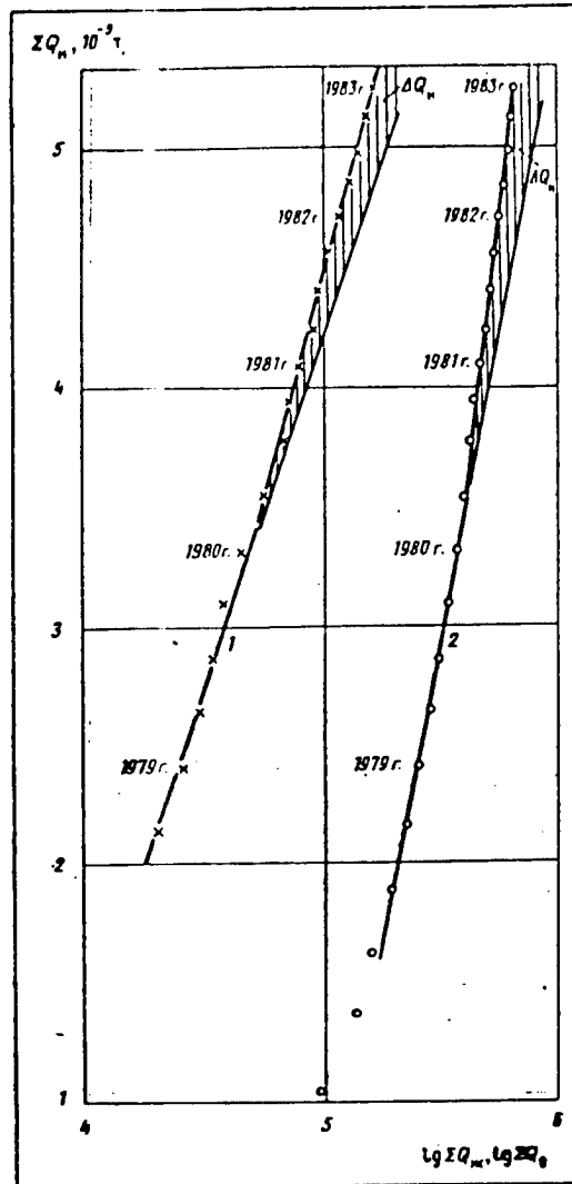
Figure 3. Characteristics of Oil Displacement from the Zone of Wet In Situ Combustion: 1 - \Sigma Q_m = f(lg \Sigma Q_m) ; 2 - \Sigma Q_m = f(lg \Sigma Q_m) ; \Sigma Q_m , \Sigma Q_o , \Sigma Q_m - total extraction of oil, water and fluid respectively
