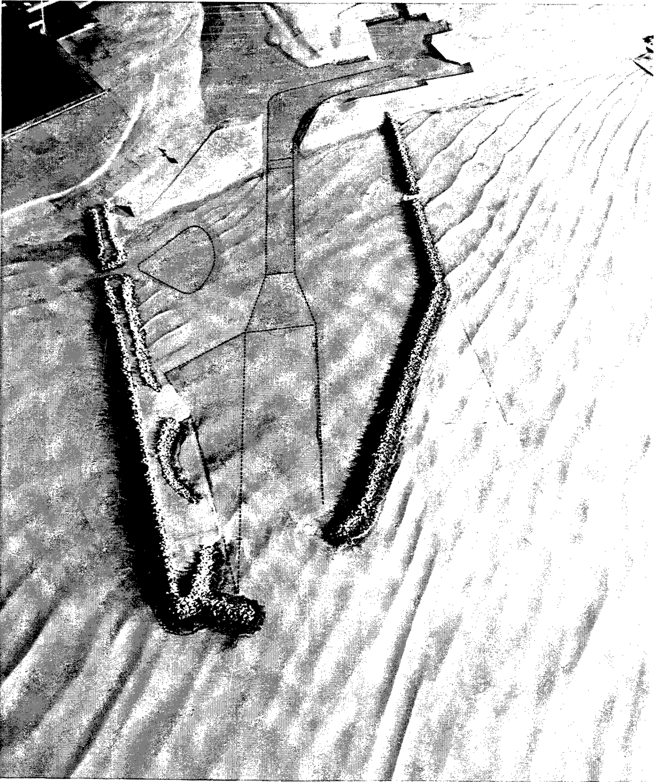
Photo 7. Typical wave patterns for Plan 19; 9-sec, 2-m (6.6-ft) waves from 137 deg; swl = +0.5-m (+1.6-ft)
