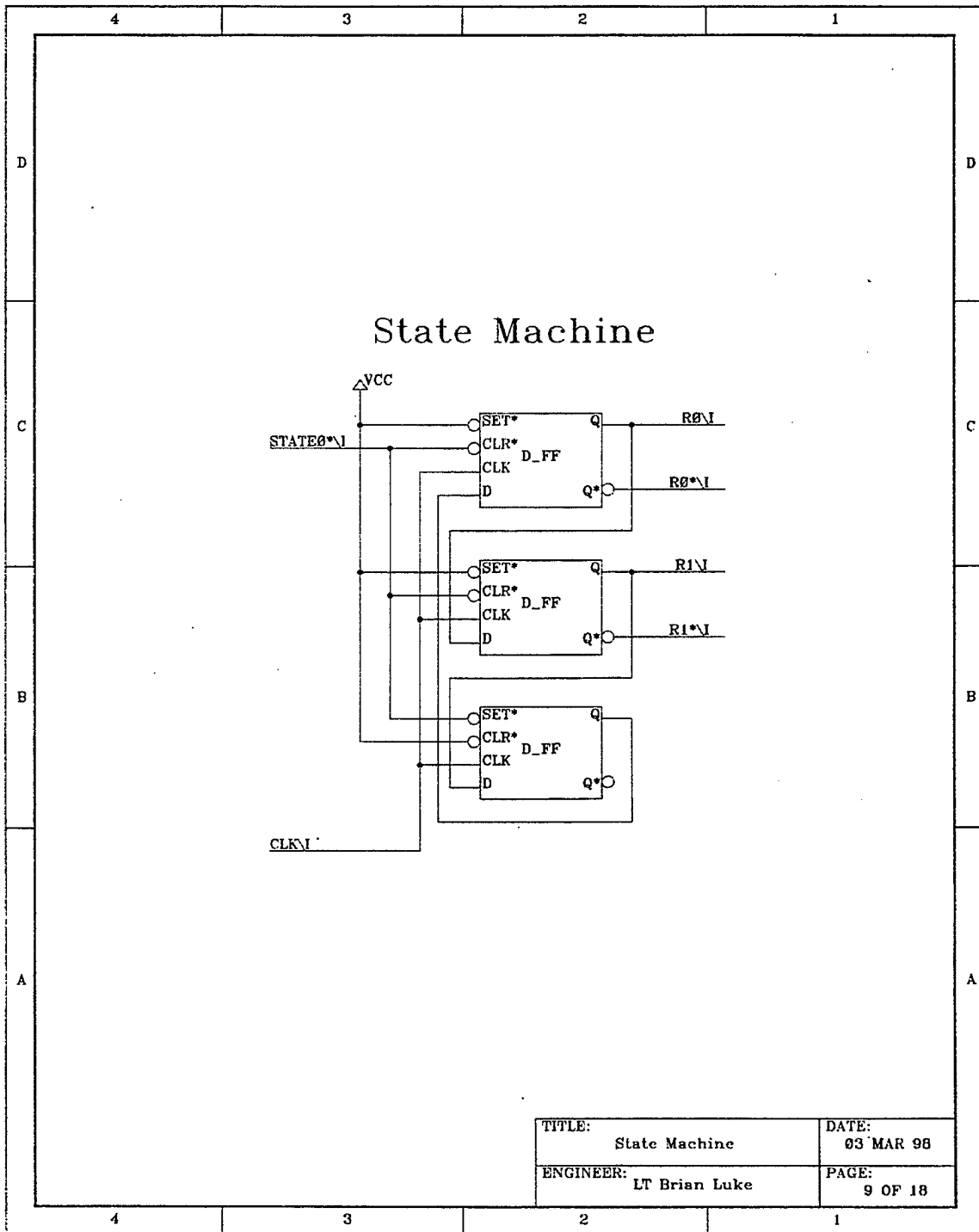
Figure 37. State Machine
