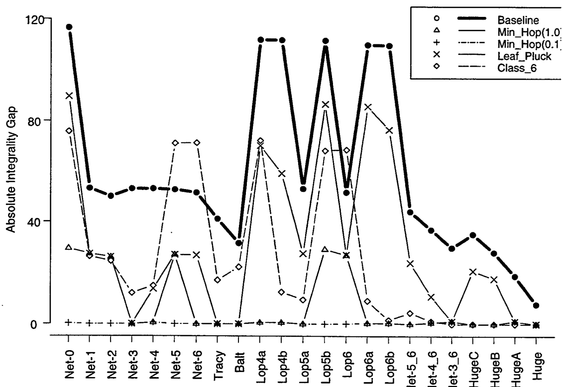
Figure 11. Effect of Preprocessing on the Relaxed Objective Function Value
