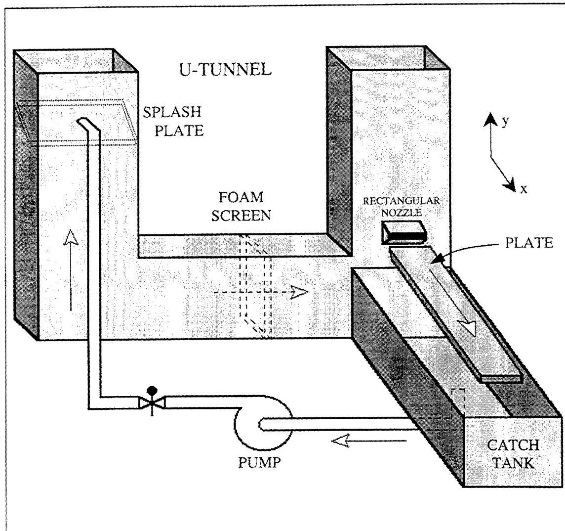
Figure 10. Equipment arrangement for the rectangular liquid wall jet experiments. The fluid flow path is as indicated by the arrows.
