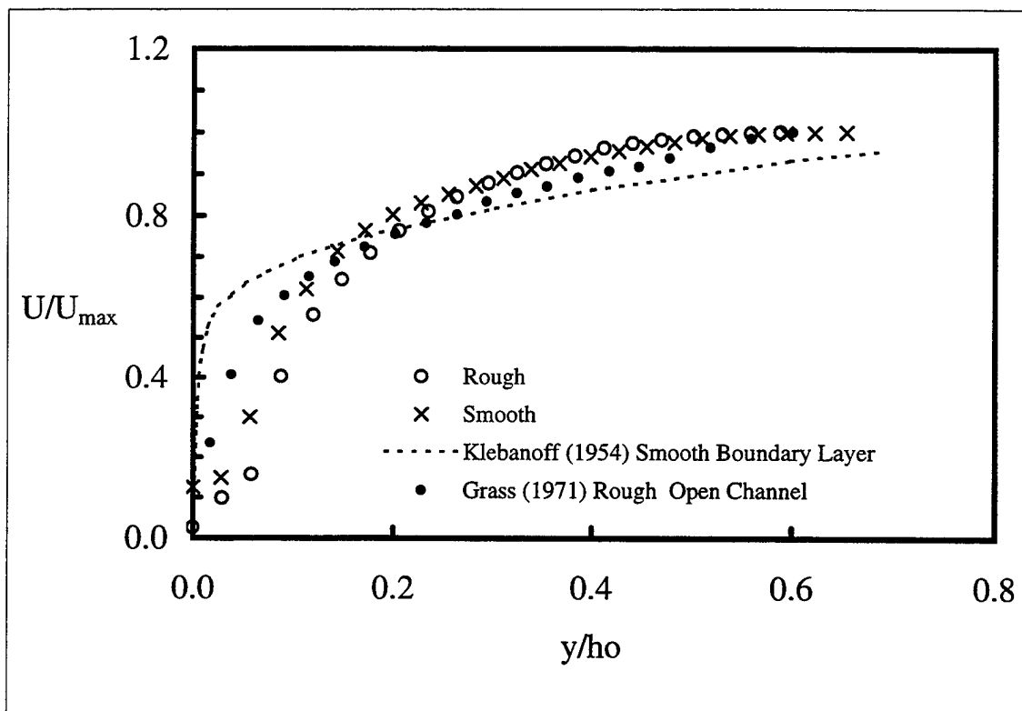
Figure 61. Mean velocity distribution across the liquid wall jet formed in the recirculating free-surface water tunnel at x/h_o = 53 .
