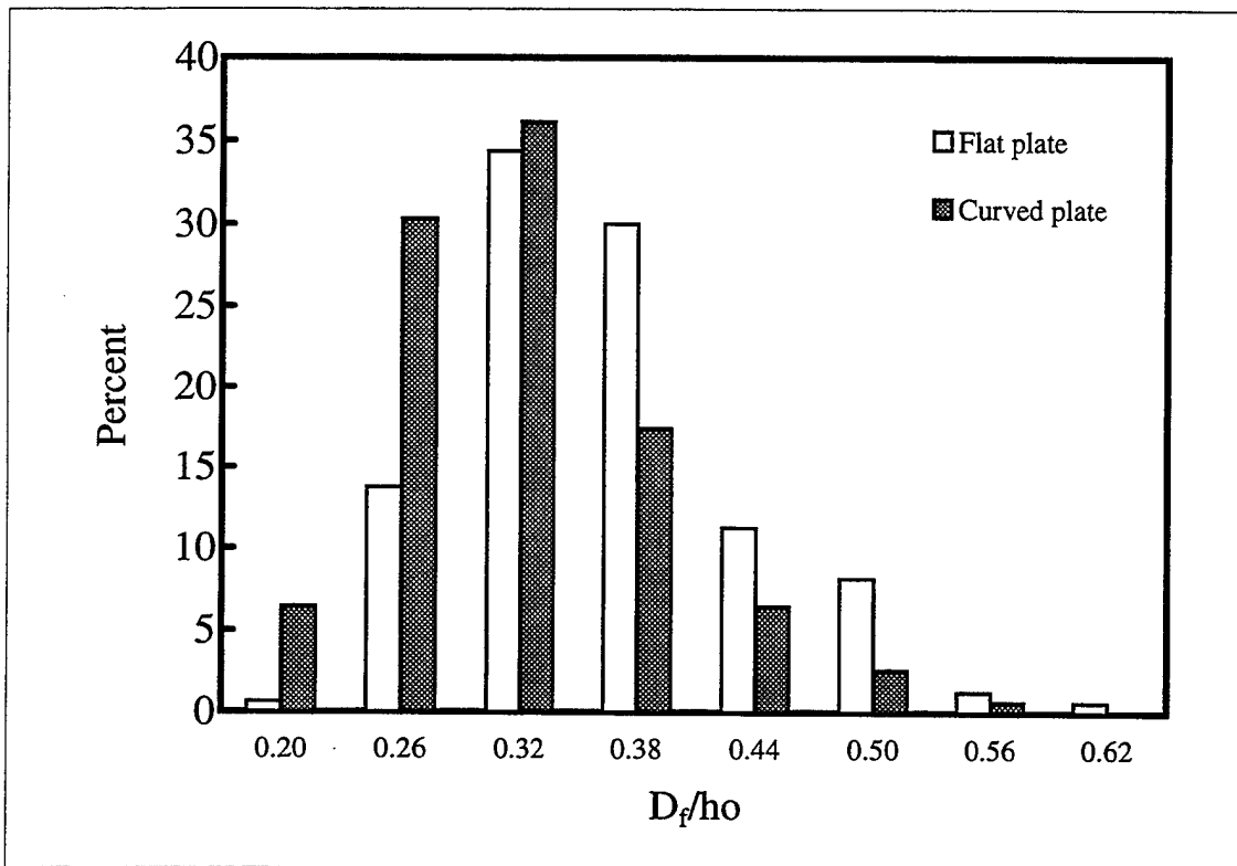
Figure 41. Distribution of the normalized effective filament diameter for the flat- and curved-wall ( k/h_o = 0.06 , We = 3000 ).
