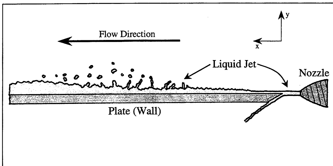
Figure 7. Diagram of a liquid wall jet.
