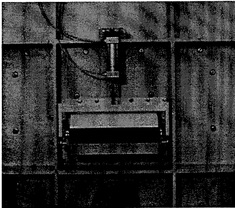
Figure 12. Photograph of the outside of the rectangular nozzle with the cylindrical gate closed.
