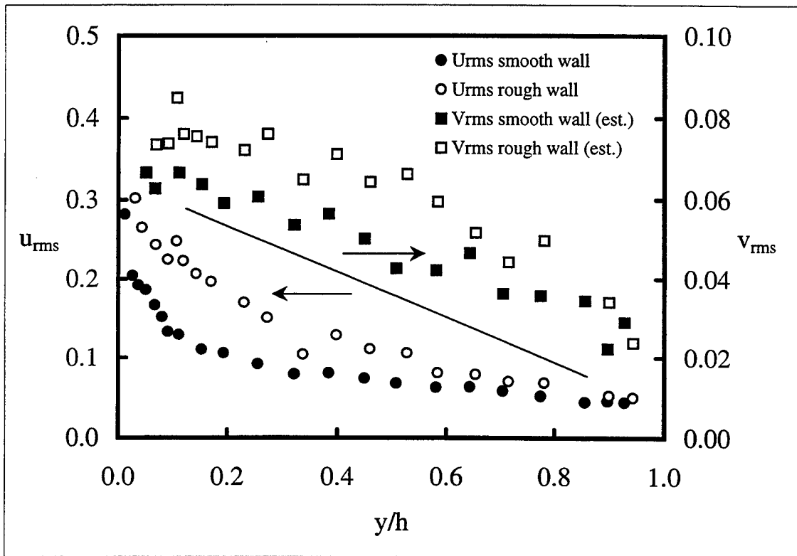
Figure 6. Streamwise and vertical turbulence intensity across a smooth- and rough-walled open channel. Re = 9800 , Fr = 0.2 . For the rough wall, k/h = 0.065 . From Nezu and Nakagawa (1993).
