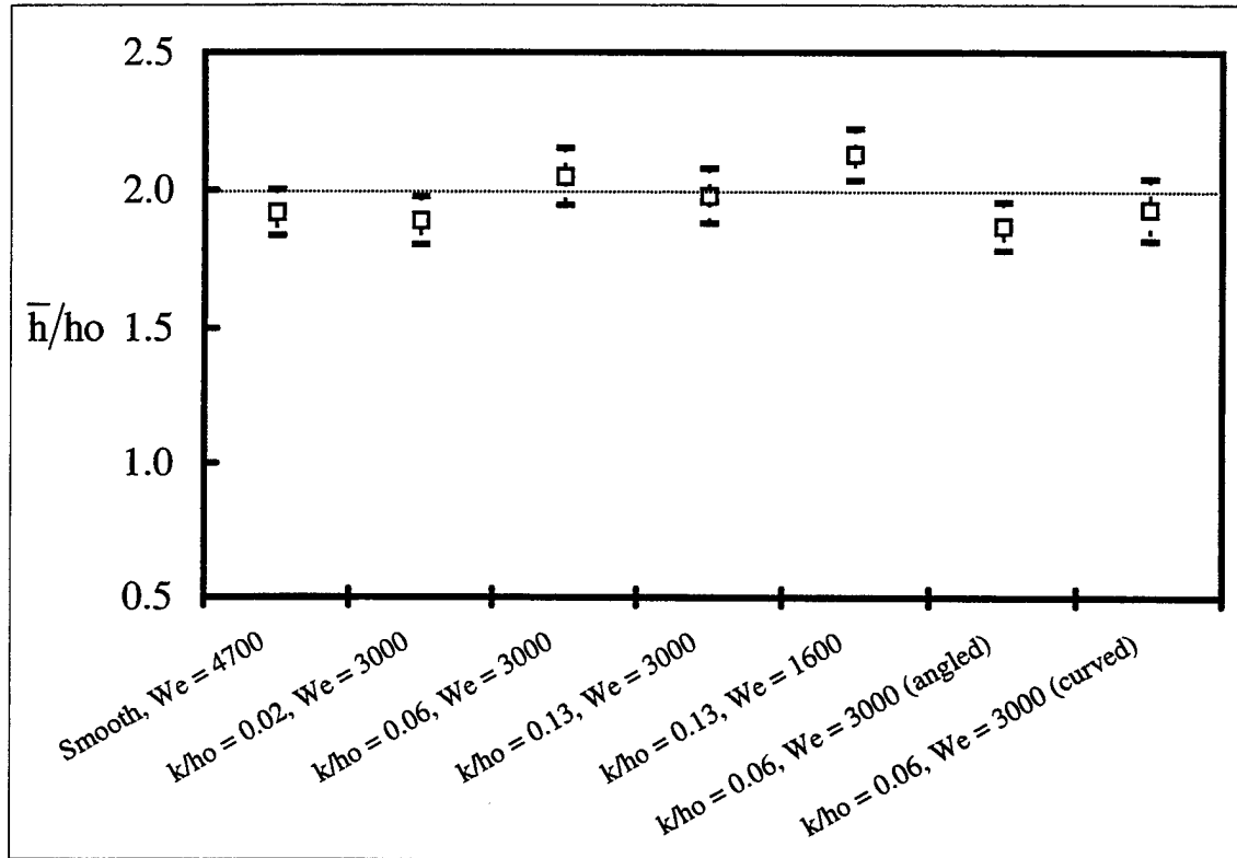
Figure 25. Normalized mean jet thickness at the beginning of the drop generation region. Uncertainty regions are bracketed and the average value is 2.0.
