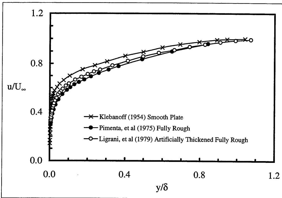
Figure 2. Mean velocity distribution across the turbulent boundary layer formed by smooth- and rough-walled surfaces.
