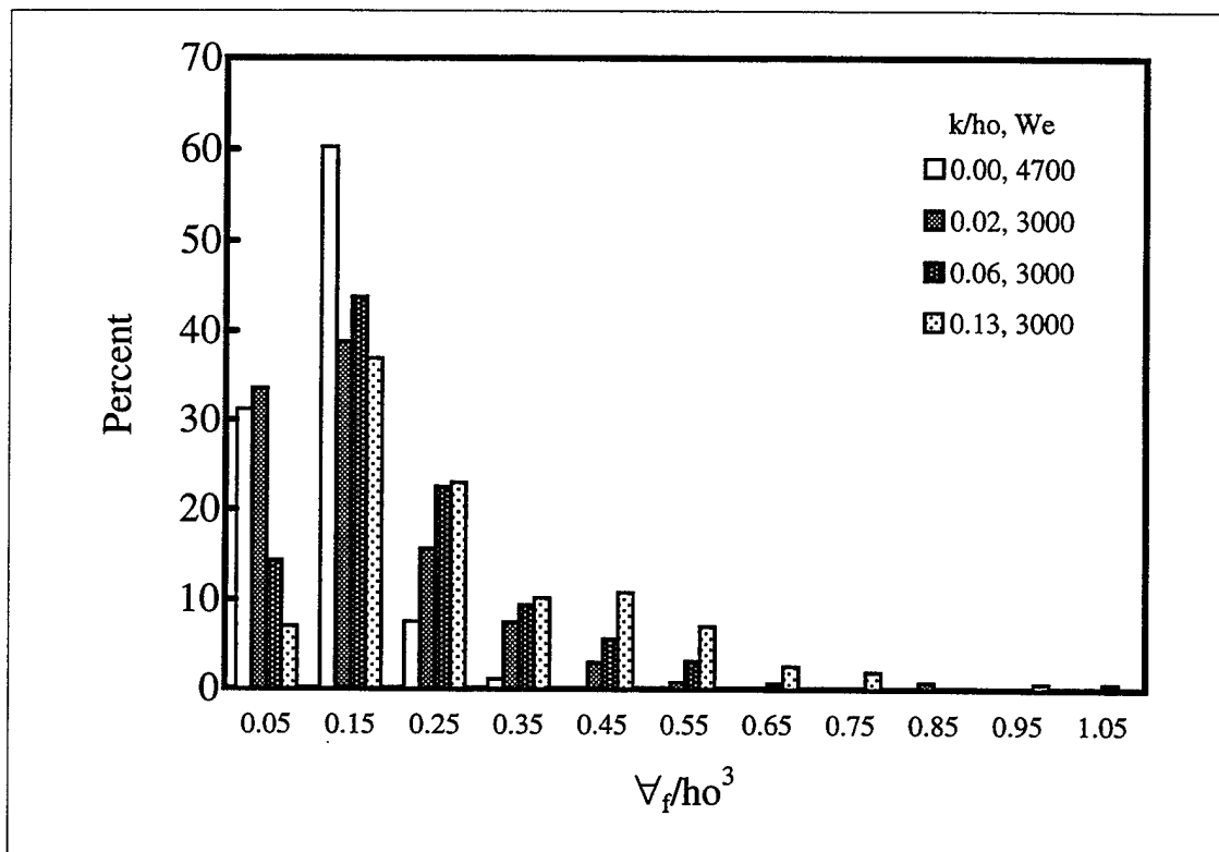
Figure 47. Distribution of the normalized filament volume as a function of the relative roughness.
