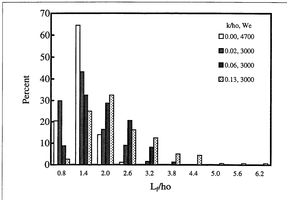
Figure 33. Distribution of the normalized filament length as a function of the relative roughness.
