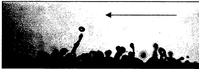
Figure 17. An image of the free surface profile of the rectangular liquid wall jet. Re_x = 2.3 \times 10^6 , Re = 3.6 \times 10^4 , Fr = 26 , We = 3000 , k/ho = 0.06 .
