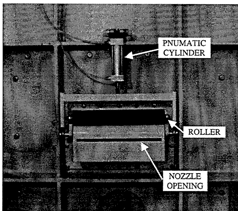
Figure 11. Photograph of the outside of the rectangular nozzle with the cylindrical gate open.
