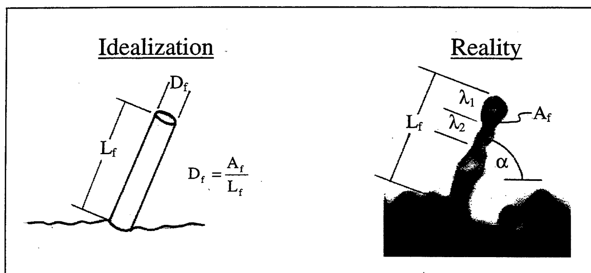
Figure 20. Diagram showing how the filament characteristics are simplified for statistical analysis.
