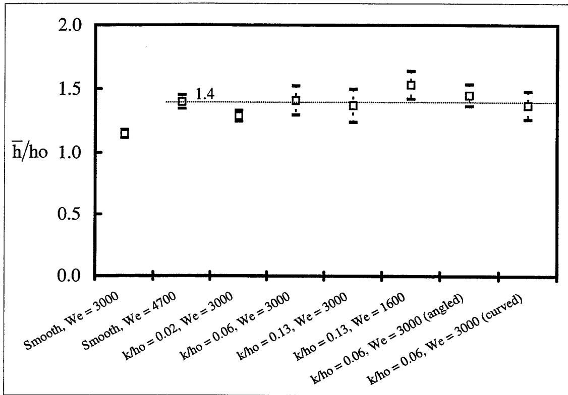
Figure 23. Normalized mean jet thickness at the beginning of the transition to roughness region. Uncertainty regions are bracketed and the average value for the drop producing runs is 1.4.
