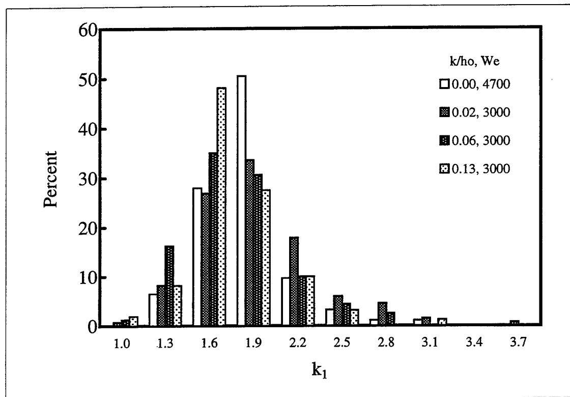
Figure 52. Distribution of the disturbance wave number as a function of relative roughness.
