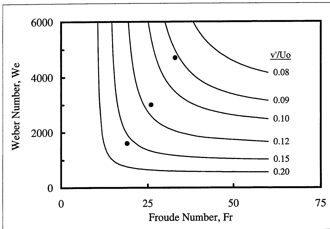
Figure 69. The jet Weber number versus the jet Froude number for different levels of v'/U_o as estimated by Eq. (10). The circles mark the three combinations of We-Fr examined in this investigation.
