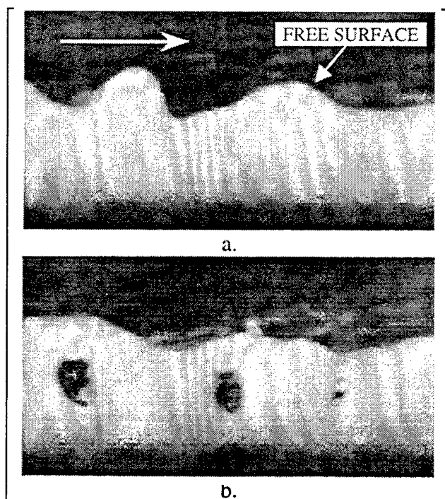
Figure 63. Two images depicting the free surface distortions and bubbles that are present in the rough-wall jet formed in the recirculating water tunnel.
