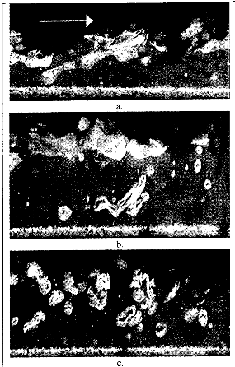
Figure 62. Photographs of the interior of a rough-wall liquid jet formed in the recirculating water tunnel. Re_x = 2.3 \times 10^6 , Re = 2.8 \times 10^4 , Fr = 9 , We = 1100 , k/ho = 0.08 .
