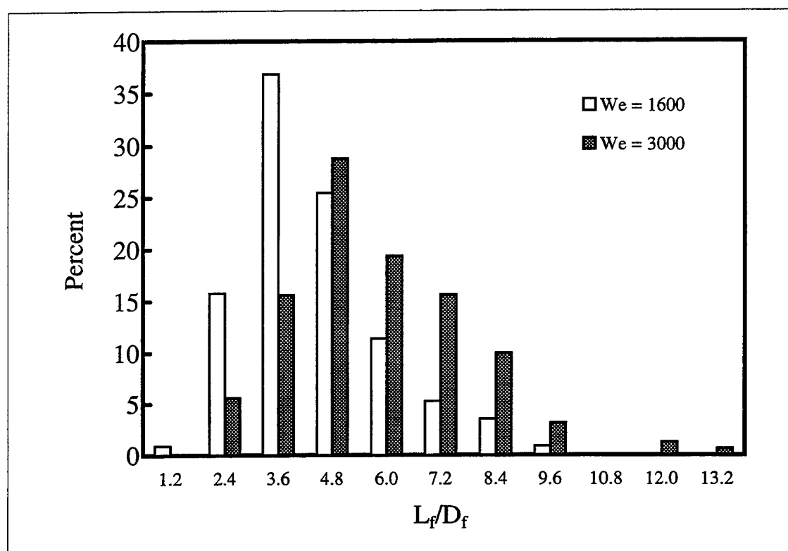
Figure 44. Distribution of the normalized filament slenderness ratio for the coarse-wall ( k/h_o = 0.13 ) at high- and low-Weber number.
