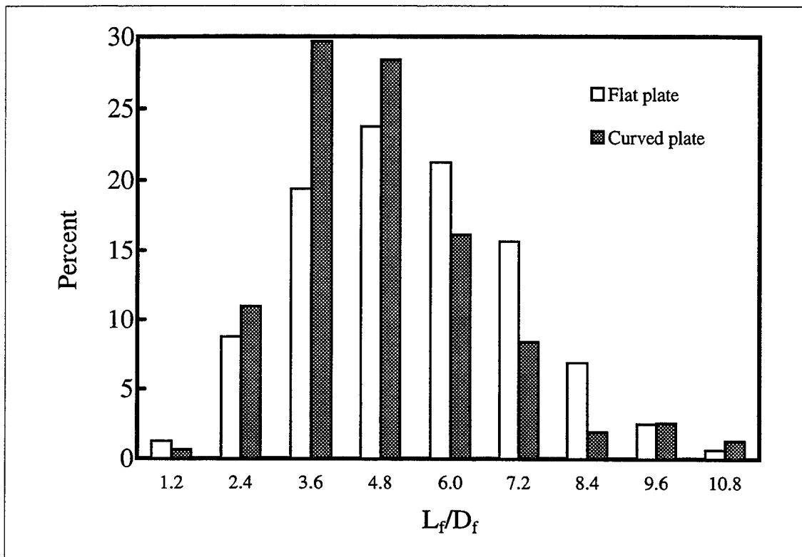
Figure 45. Distribution of the normalized filament slenderness ratio for the flat- and curved-wall ( k/h_o = 0.06 , We = 3000 ).
