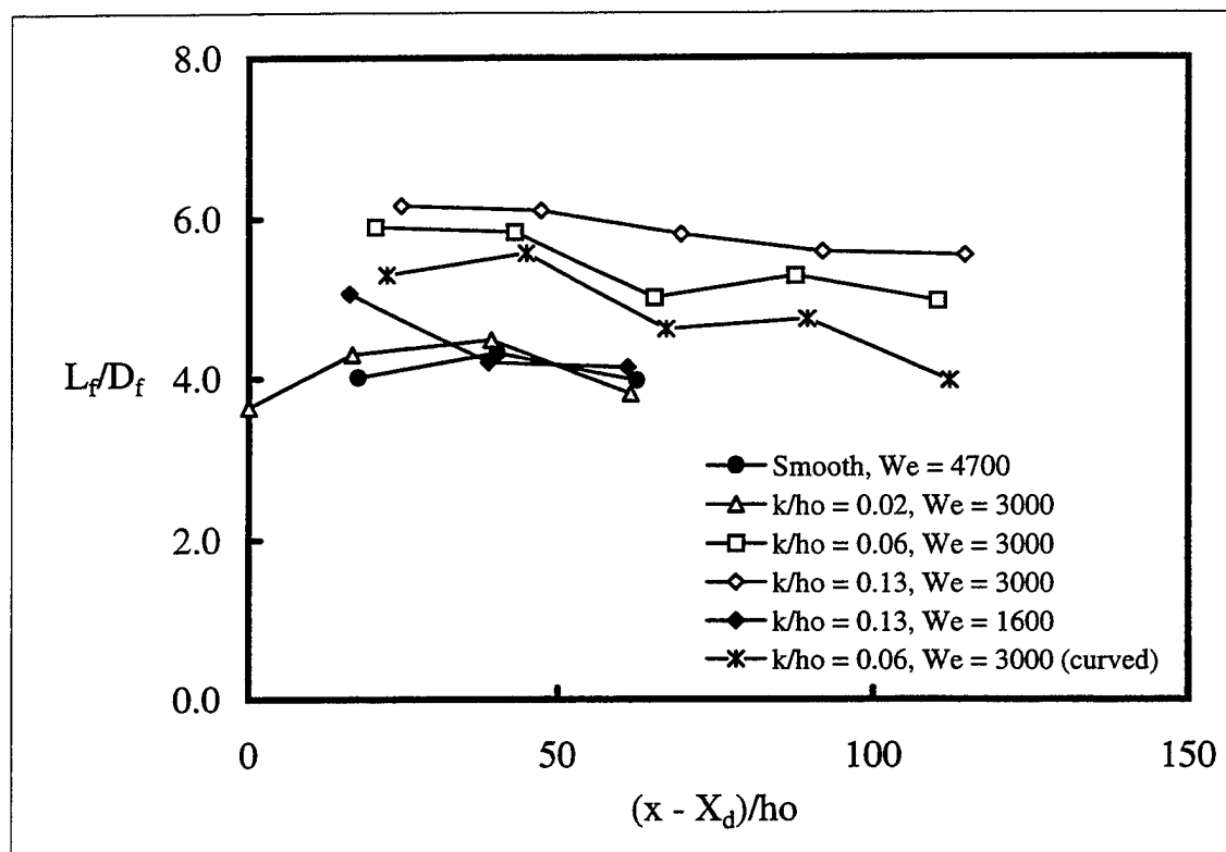
Figure 58. Normalized mean filament slenderness ratio as a function of the nondimensional streamwise coordinate. Here x and X_d denote, respectively, the distance from the leading edge of the plate and the point at which drop generation begins. Only those locations with >30 observations are shown. The uncertainty is approximately 15 percent.
