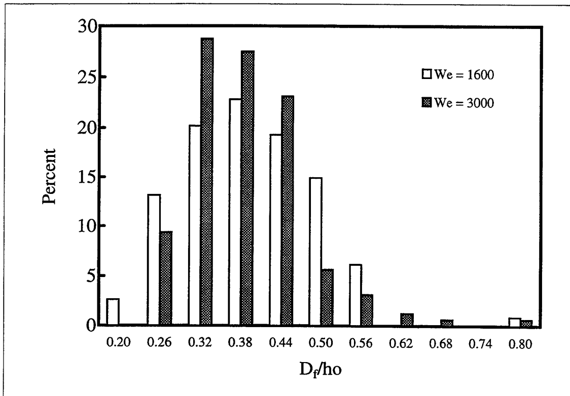
Figure 39. Distribution of the normalized effective filament diameter for the coarse-wall ( k/h_o = 0.13 ) at high- and low-Weber number.
