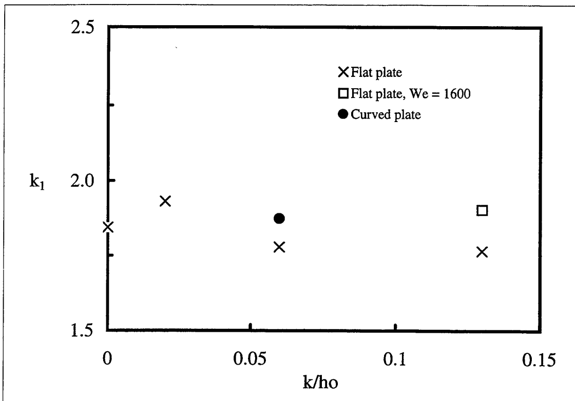
Figure 51. Mean disturbance wave number at the tip of the filament just prior to drop separation.
