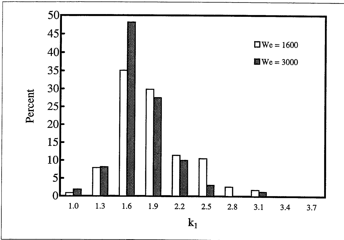
Figure 53. Distribution of the disturbance wave number for the coarse-wall ( k/h_o = 0.13 ) at high- and low-Weber number.
