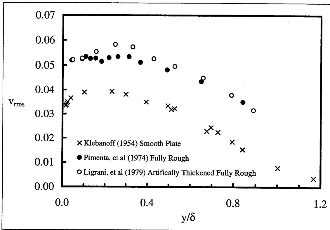
Figure 4. Vertical turbulence intensity across the boundary layer formed by smooth- and rough-walled surfaces.
