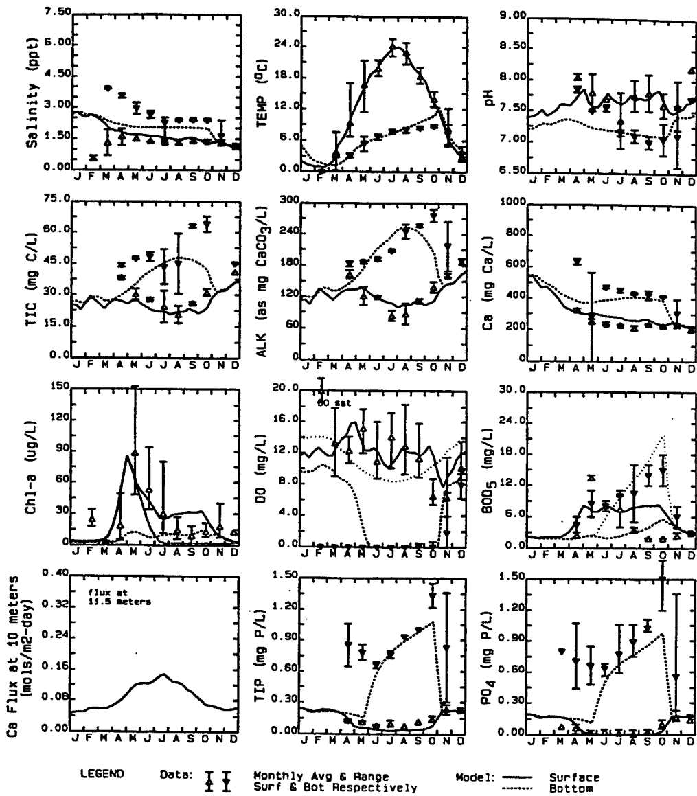
Fig. 8.3 Calibration results for RCA water quality model for 1986. Monthly averages for surface layer: model (solid line), data ( \Delta ) \pm range; and bottom layer model (dotted line), data ( \nabla ) \pm range.
