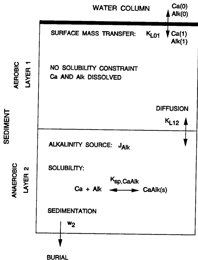
Fig. 4.1 Schematic diagram of the calcium and alkalinity flux model.
