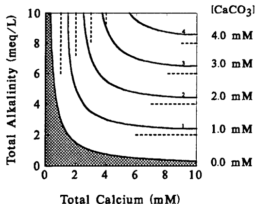
Fig. 4.2 Concentration of CaCO_3(s) as a function of total alkalinity and total calcium concentrations. CaCO_3 = 0 in the shaded region. The dotted lines are the stoichiometric limits to the quantity of CaCO_3(s) that can form as Ca_T or Alk_T \rightarrow \infty .
