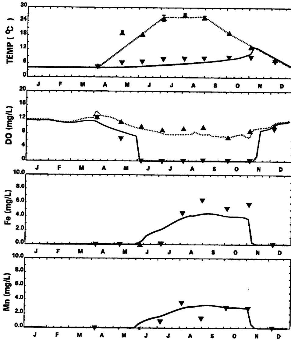
Fig. 9.3 Croton resevoir site 5 iron and manganese calibration, 1993.
