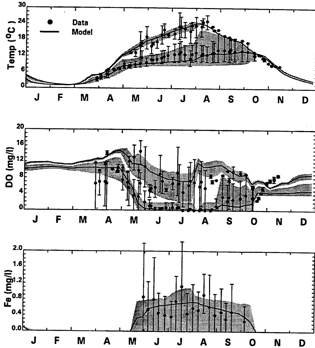
Fig. 8.10 Calibration results for Onondaga Lake. Temporal results, 1988.
