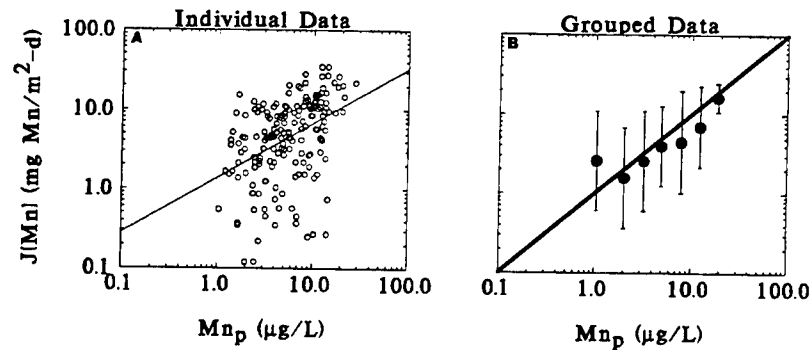
Fig. 7.3 (A) The observed manganese flux J[Mn] versus the particulate manganese concentration in the overlying water Mn(0)_p . Only data for which Mn(0)_p > 1\mu\text{g/L} are included in order to reduce the influence of analytical errors at low concentrations. The linear regression line is shown. (B) The data are grouped in 0.2 \log_{10} units. The mean \pm the standard deviation is shown. The line corresponds to a settling velocity of w_1 = 1 m/d.
