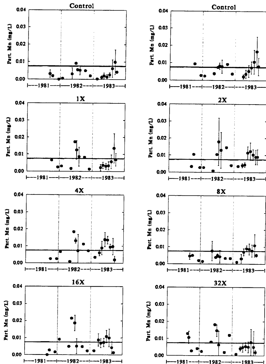
Fig. 5.9 Particulate concentrations in the overlying water. Line is the concentration used in the model for the depositional flux.
