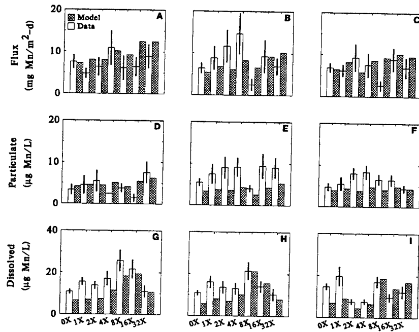
Fig. 7.10 Comparison of average annual data and model results: 1981 (A,D,G); 1982 (B,E,H); 1983 (C,F,I). Manganese flux (A,B,C). Water column particulate (D,E,F) and dissolved (G,H,I) manganese.
