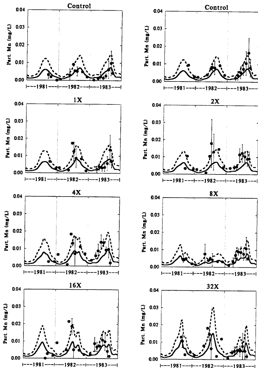
Fig. 7.12 Computed particulate MnO_2(0) (dashed line) and filterable MnO_2(0) - f_{colloidal}MnO_2(0) manganese in the water column compared to observations.
