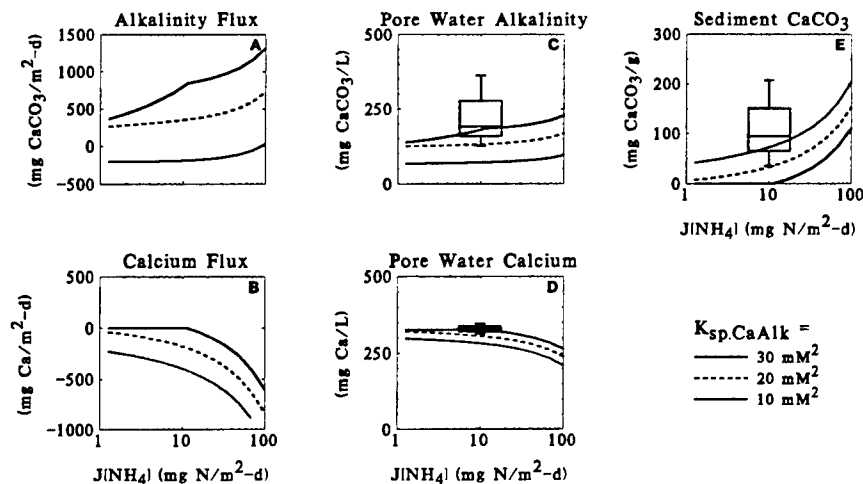
Fig. 4.4 Comparison of model results to Long Island Sound pore water data for various apparent solubility products K_{CaAlk} .
