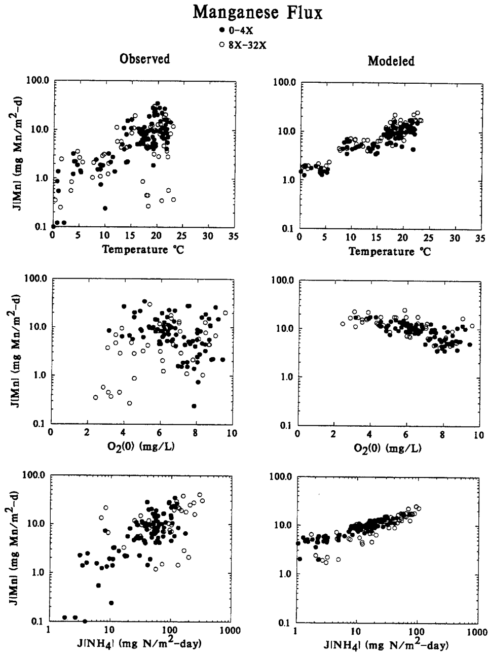
Fig. 6.7 Comparison of modeled and observed fluxes versus temperature, overlying water O 2 concentration and ammonia flux J[NH_4] .
