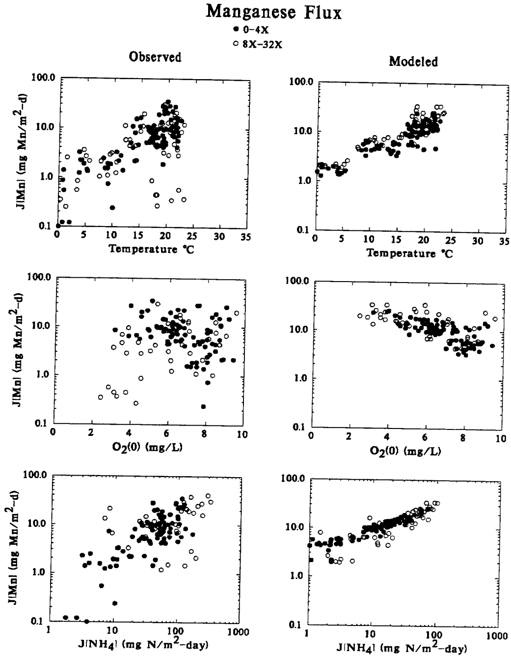
Fig. 5.11 Comparison of modeled and observed fluxes versus temperature, overlying water \text{O}_2 concentration, and ammonia flux J[NH_4] .
