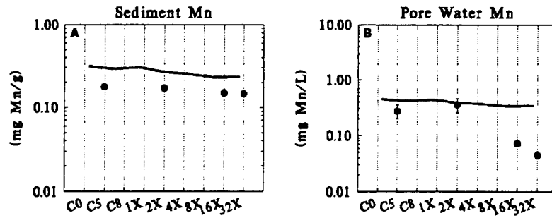
Fig. 5.7 Comparison of pore water and solid phase concentrations.
