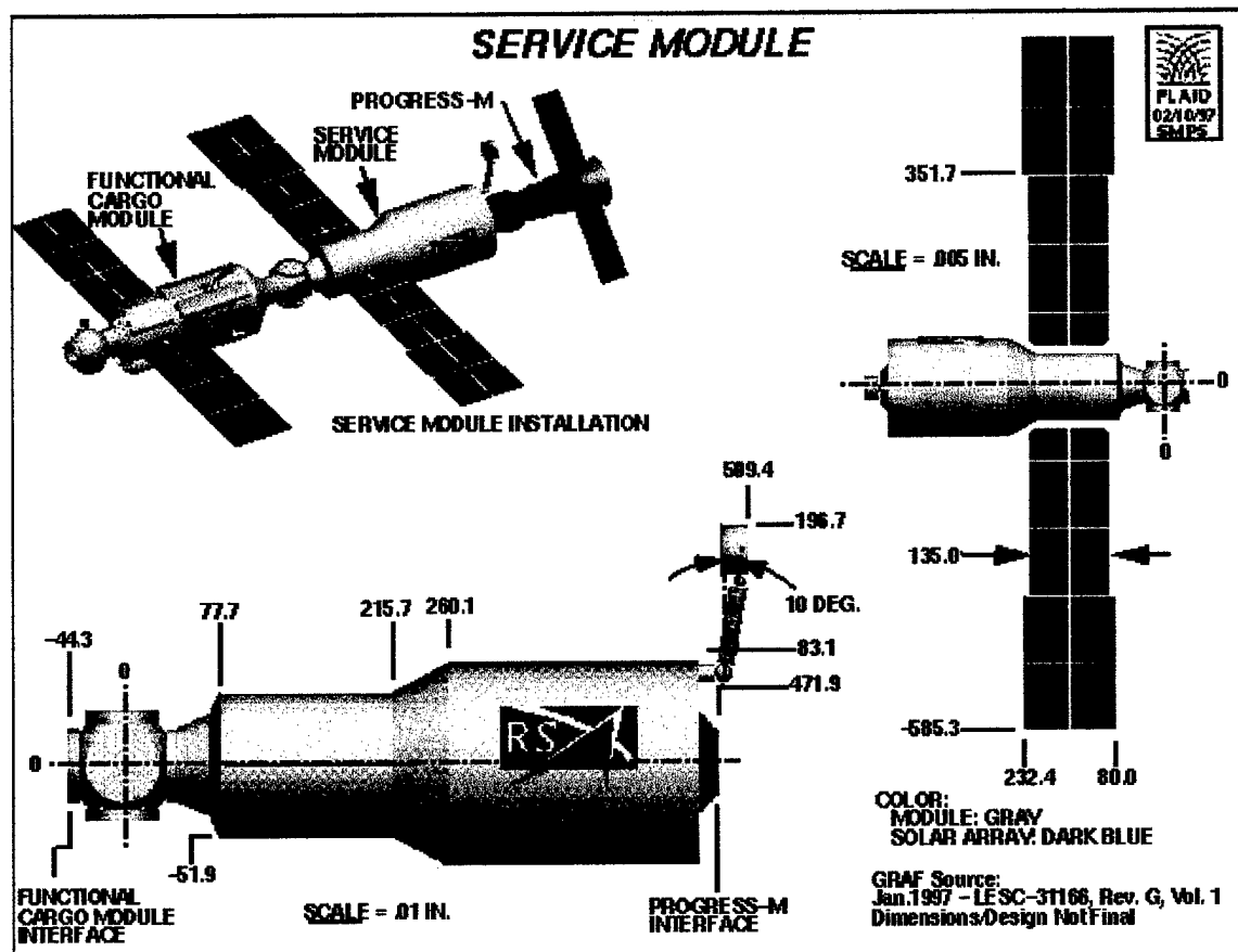
Figure 10. Another perspective of the Service Module. Note its relationship to the FGB. The Node 1 adapter joins the FGB and Service Module. The Progress M is the Russian logistics refueling and servicing spacecraft.
