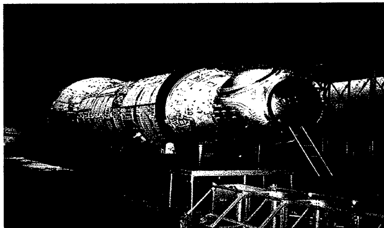
Figure 6. The Boeing-contracted, Khrunichev Productions Space Center-built, Functional Cargo Block (FGB). The FGB will be placed into orbit by a Proton launched vehicle from the Baikonur Cosmodrome.
