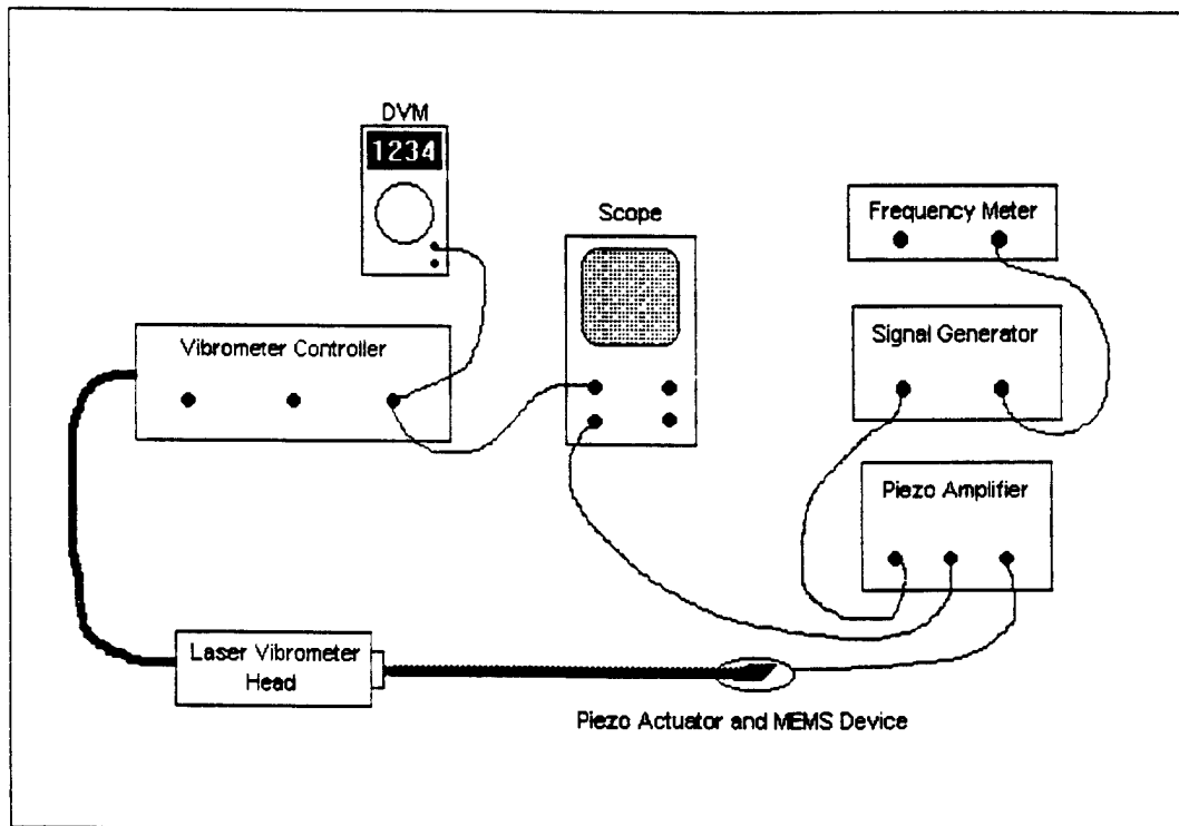
Figure 14 Test Set 2 Resonance Measurement Setup
