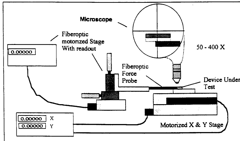
Figure 5 Graphical Description of force/displacement characterization station
