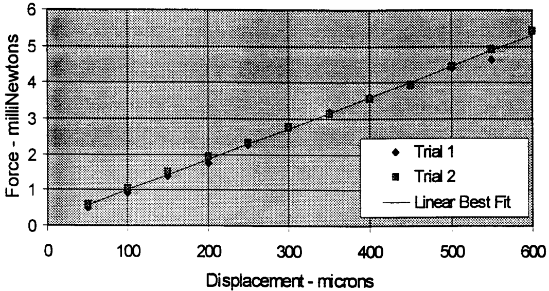
Figure 4 - Device 2B Displacement - Force Testing
