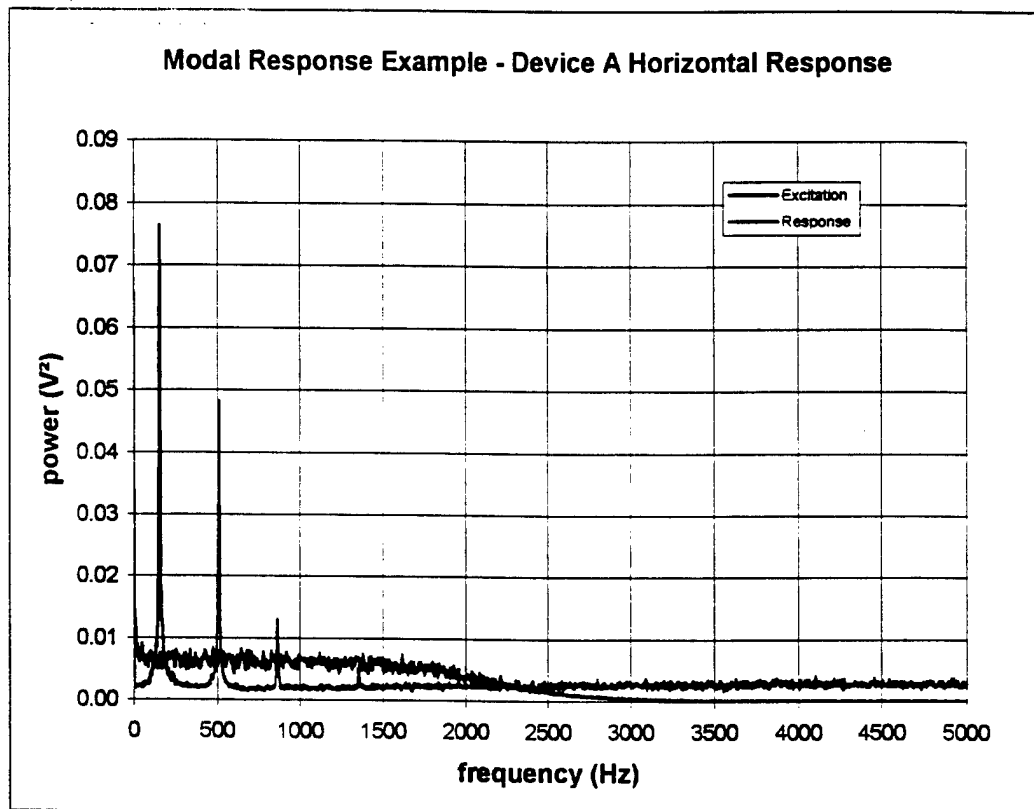
Figure 13 Modal Response Example
