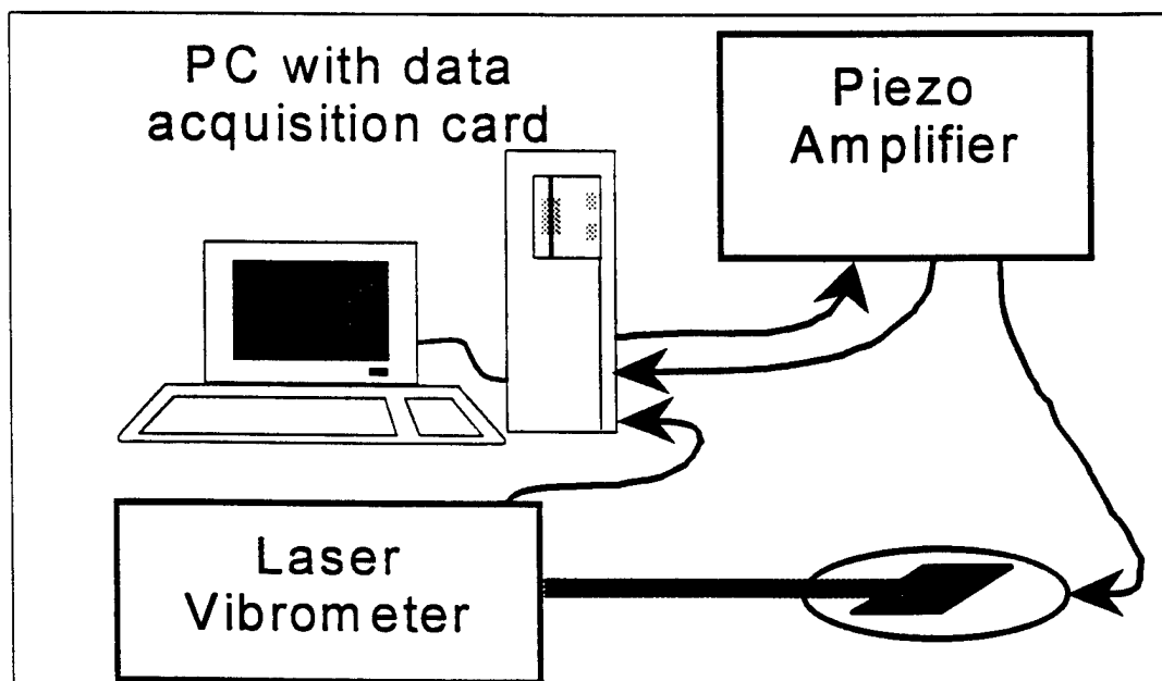
Figure 12 Test Set 1 Resonance Measurement Setup
