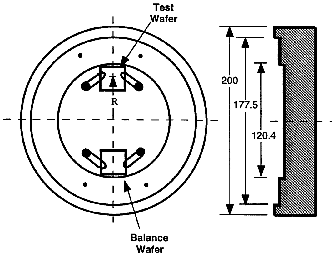
Figure 1: G sensor test fixture. Units in millimeters.
