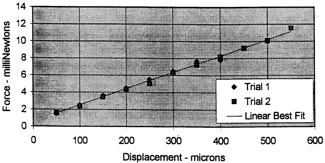
Figure 5 - Device 2C Displacement - Force Testing
