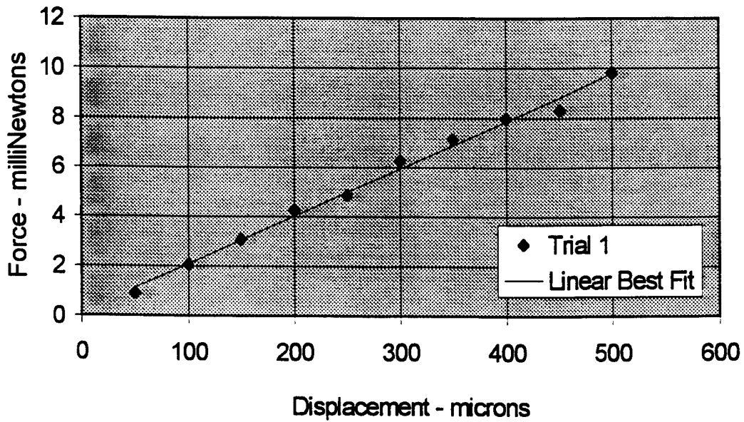
Figure 7 - Device 2E Displacement - Force Testing
