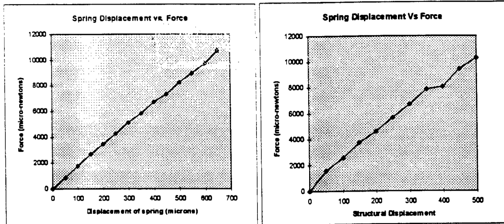
Figure 6 Measured force vs displacement of NSWC springs
