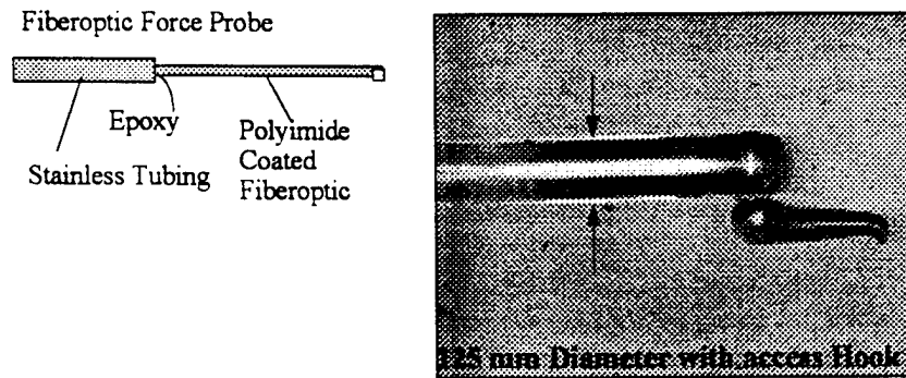
Figure 2 Picture of fiberoptic Probe (Artist) and actual probe with special tip
