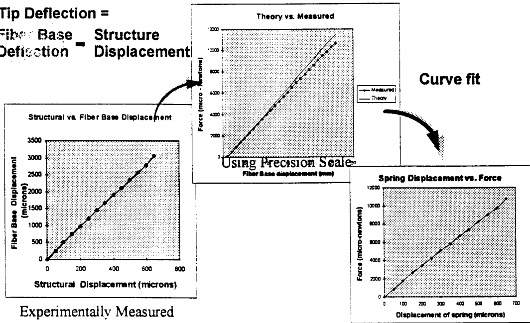
Figure 4 Schematic illustration of procedure to obtain Force vs displacement for structures
