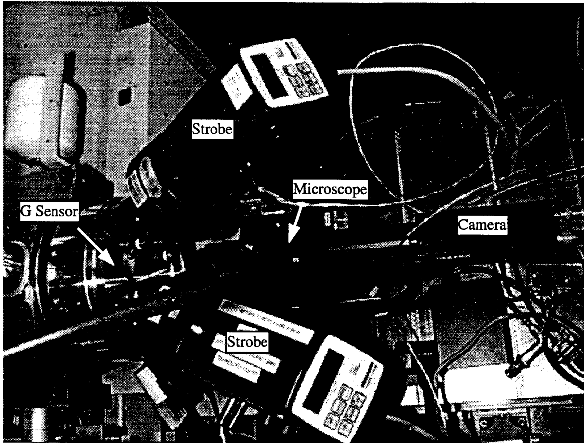
Figure 5: Top view of test setup for second round of testing.
