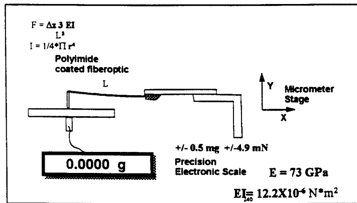
Figure 3 Graphical description of fiberoptic probe calibration setup
