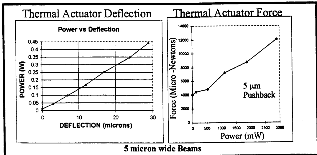
Figure 7 Thermal actuator Force / Deflection versus Power characterization curves
