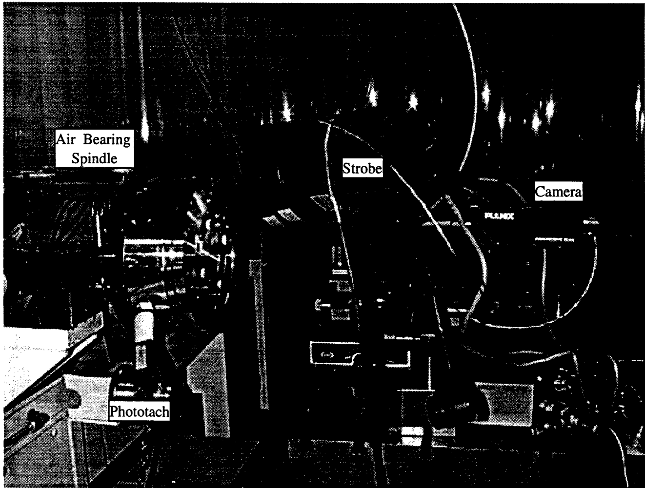
Figure 3: Nanoform 600 test setup during the second round of spin tests.
