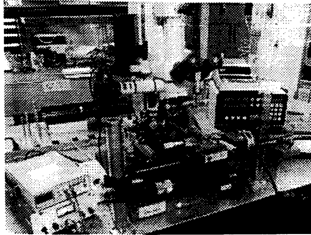
Figure 1. Picture of force and displacement characterization
