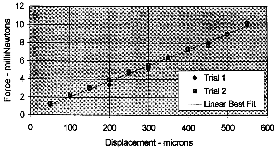
Figure 6 - Device 2D Displacement - Force Testing
