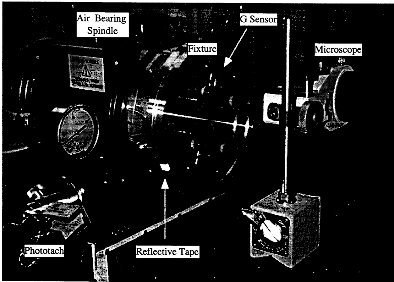
Figure 2: Setup on Precitech diamond turning machine. First round of testing. Strobe and camera are not shown in this photo for clarity.
