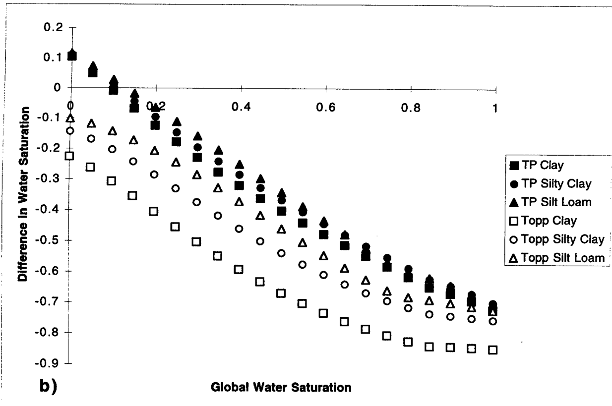
Figure 3.2. a) Difference between estimated and actual water content. b) Difference between estimated and actual water saturation. For EMT perpendicular to propagation for sand-fine systems at a 0.50 fine fraction.
