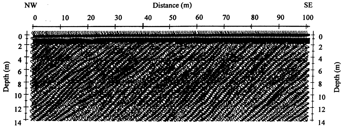
Figure 2.5. GPR profile collected over the fan-foreset delta (modified from Smith and Jol, 1992a).
