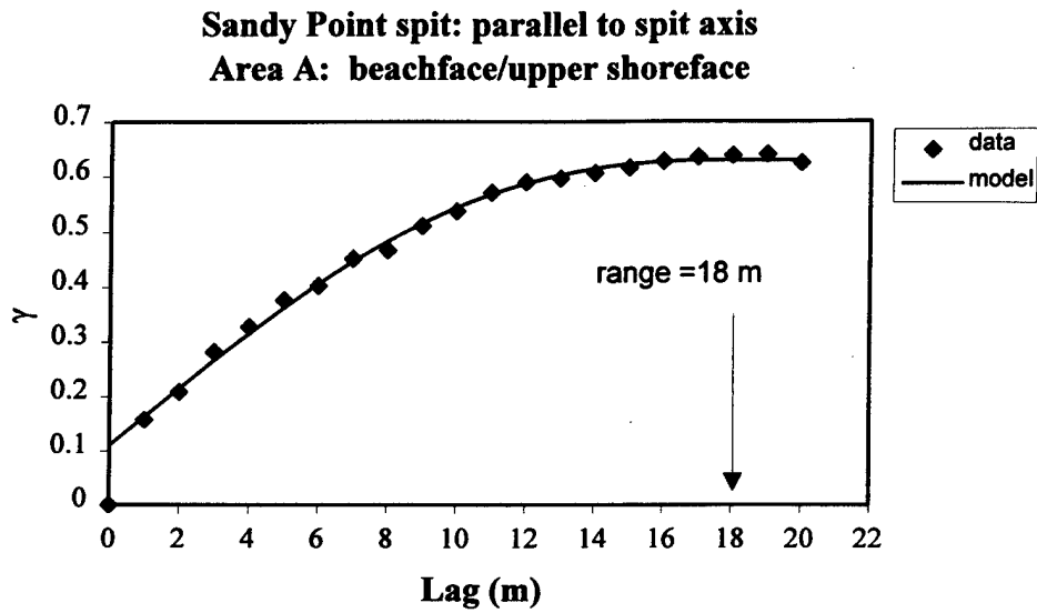
Figure 2.10a. Semivariogram analysis of area “A” in Figure 2.9. These data are modeled using a pentaspherical model with a range of 18 m.
