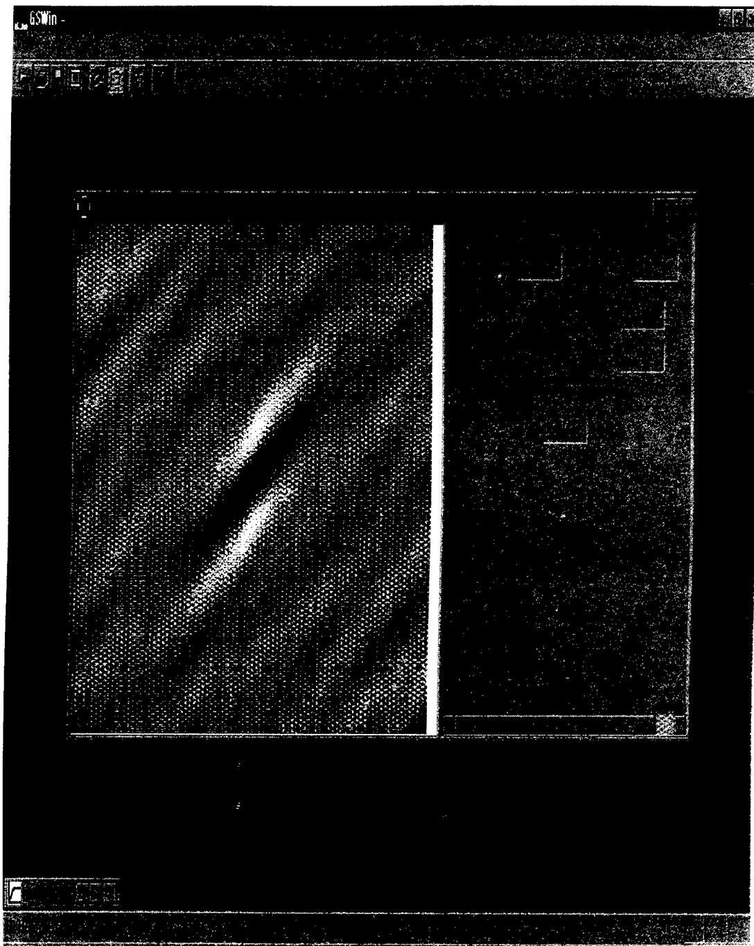
Figure 2.3. Two dimensional variogram. The angle of the dark ellipse indicates the maximum correlation direction.
