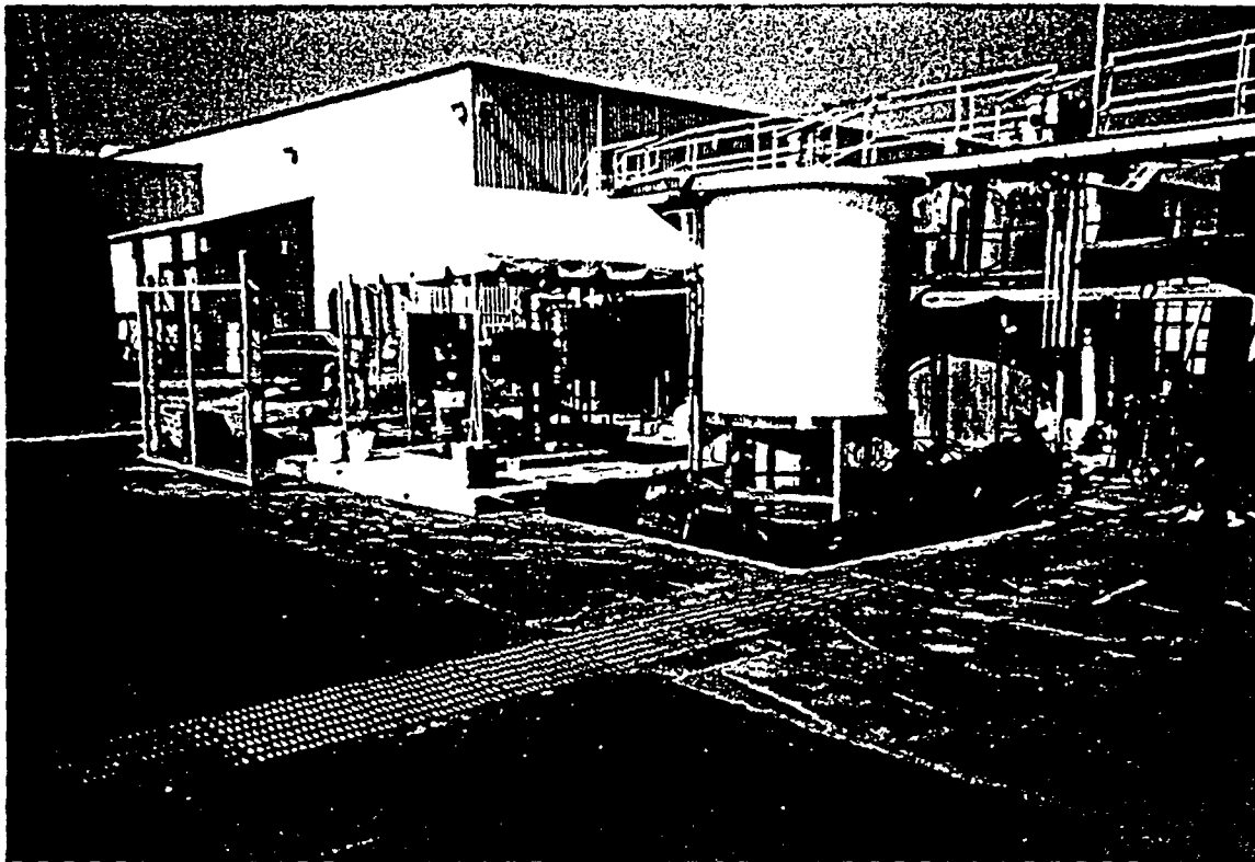
Figure 3. Photograph of the Test Facility Showing the 1000-Gallon Sludge Holding Tank.
