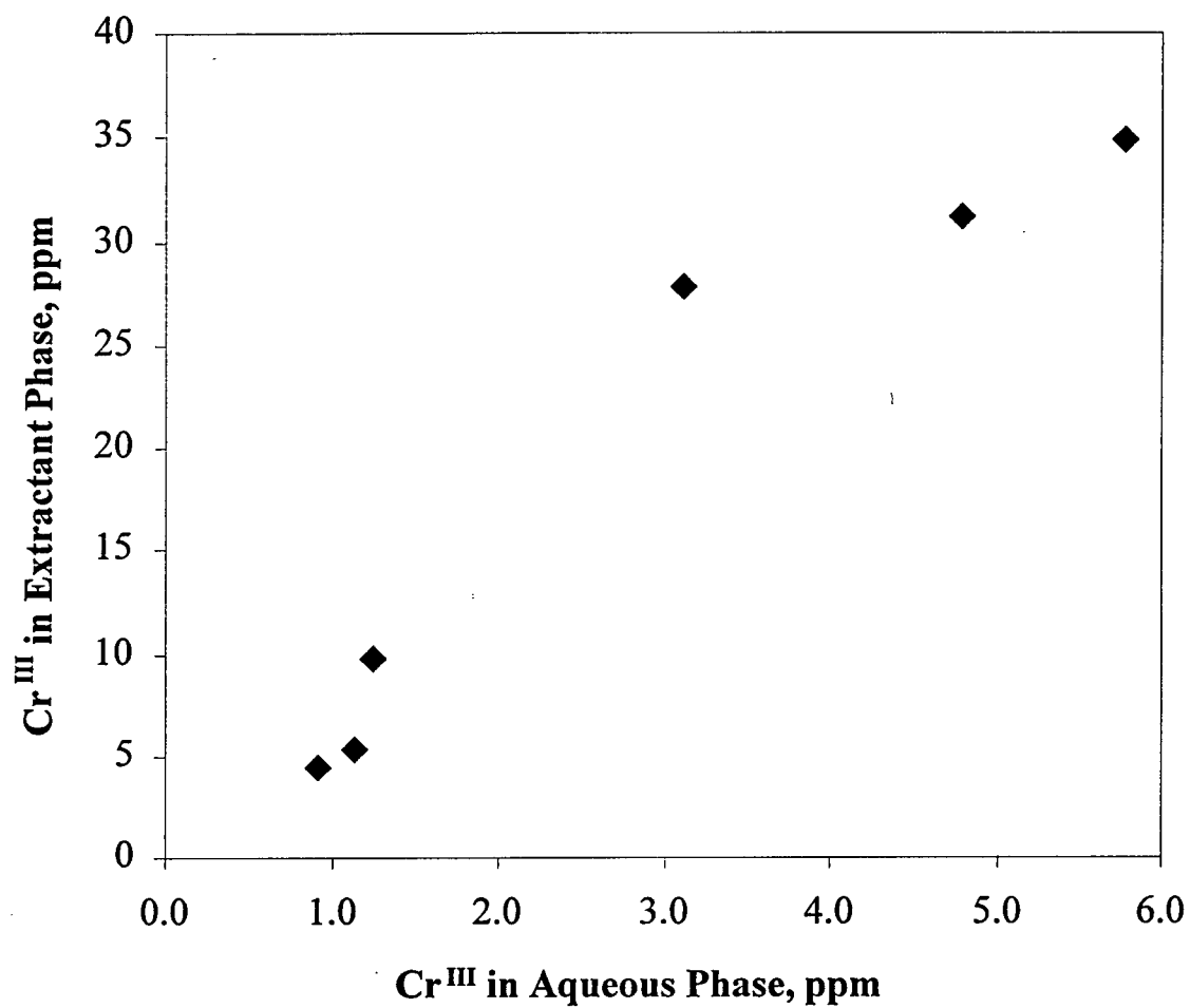
Figure 20. Comparison of the \text{Cr}^{\text{III}} Accumulation in the Aqueous and Extractant Phases of the Second Stripping Stage.
