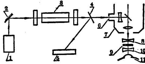
Figure 1. Optical path of the 694.3 ruby laser
