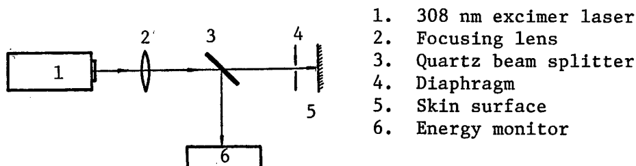
Fig. 1. Schematic diagram of the experimental setup
