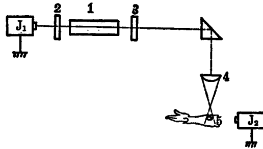
Figure 1 1--Nd glass; 2,3--Reflection mirrors; 4--Focusing lens (f/45); 5--Skin to be irradiated; J 1 --Real time energy monitor; J 2 -- Energy meter for output beam
