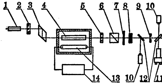
Figure 1. Q-switched frequency doubled YAG laser setup
