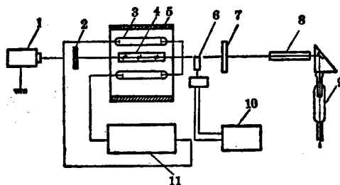
Figure 1. Schematic diagram of the Nd 3+ :YAG laser
