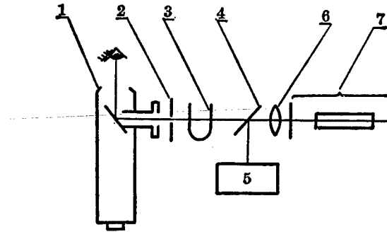
Figure 2. Schematic diagram of the optical path
