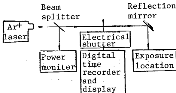
Figure 1. Experimental setup
