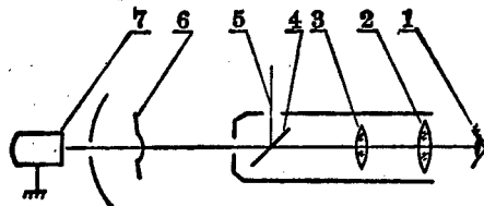
Figure 1. Optical path used in measuring the transmissivity of the rabbit eye
