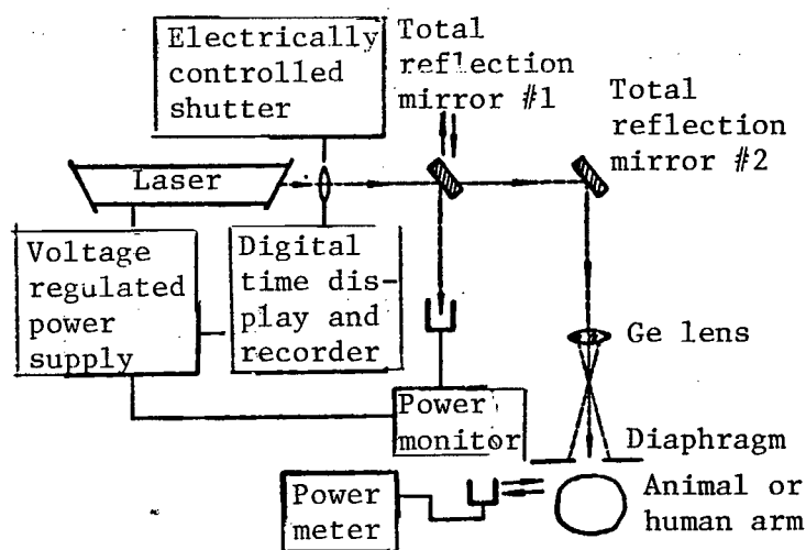
Figure 1. Experimental setup
