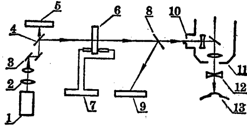
Figure 1. Optical path for retina irradiation by 488 nm argon ion laser
