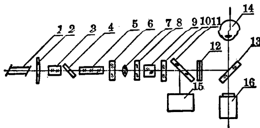
Figure 2. Optical path of the experimental setup
