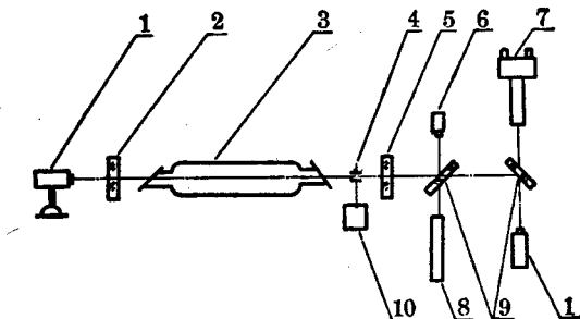
Figure 1. Optical system used in the experiment
