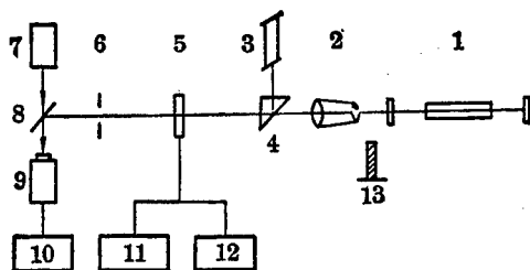
Figure 2. Optical path for CW Nd 3+ :YAG laser output power measurement
