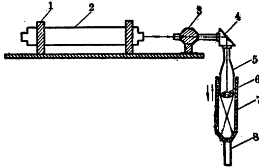
Figure 1. Optical transmission system
