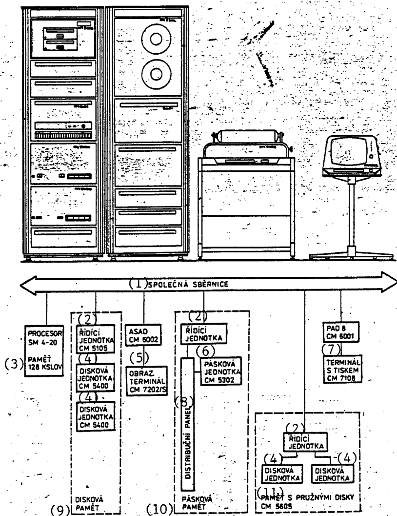
Figure 2. SM 4-20 microcomputer (variant 2/4)
