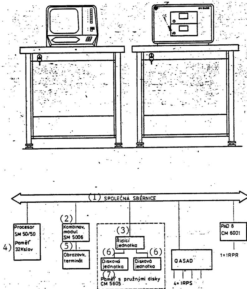
Figure 4. SM 50/50 terminal station
