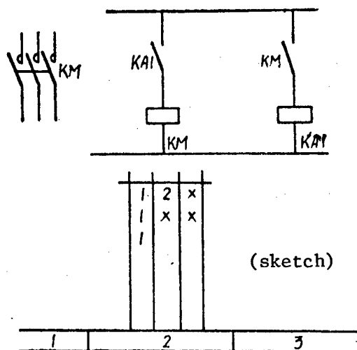
Figure 16. Tabular Representation of Components (Contacts)
