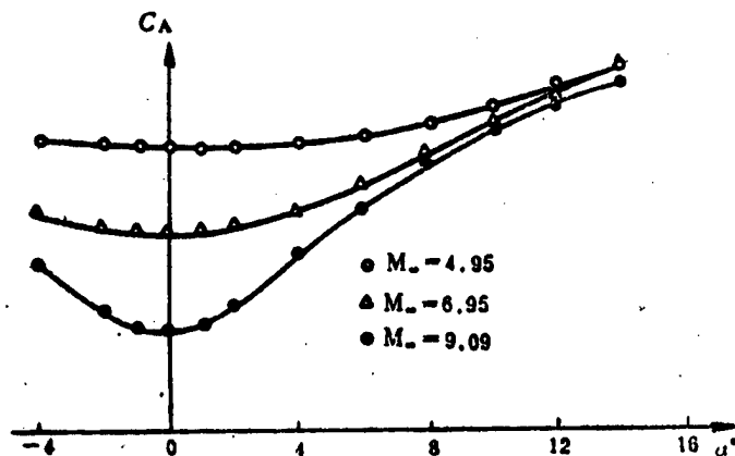
Fig. 8. Axial Force Coefficient of Recovery Body Under Sidewise Jettison- Drag Cone Scheme in Hypersonic Wind Tunnel With Changes in the Angle of Attack
