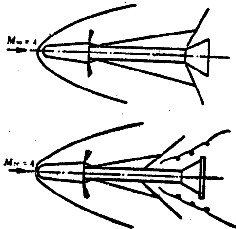
Fig. 3. Flow Diagram of Sidewise Jettison-Drag Cone in Hypersonic Wind Tunnel
