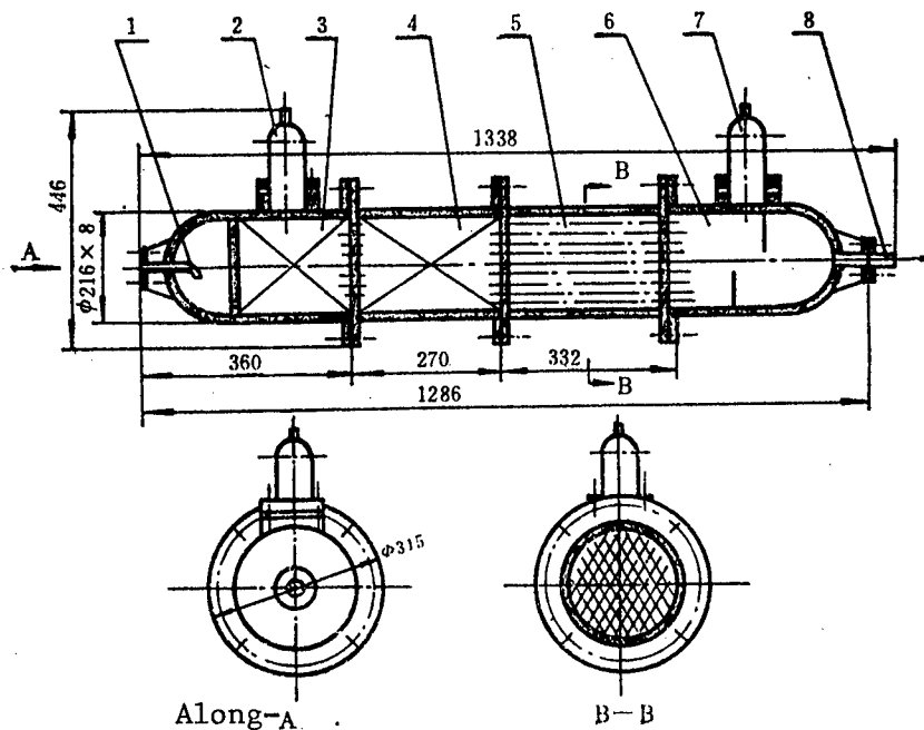
Figure 4. Coalescer Structure
