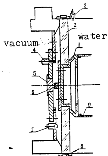
Figure 5. Construction of the diode tube
