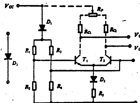
Figure 1. Typical circuitry of integrated pressure transducer
