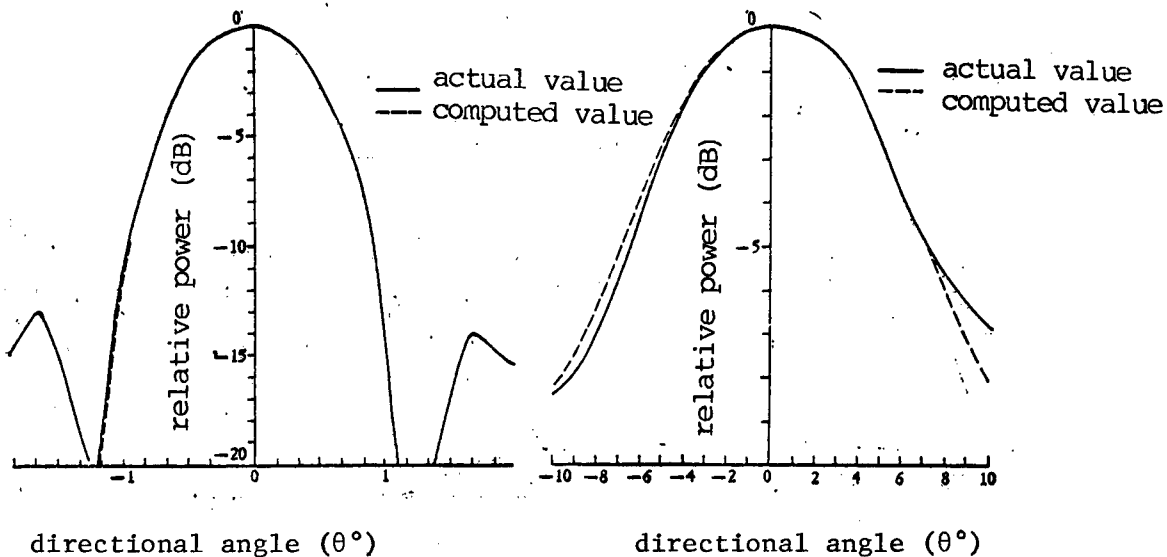
Figure 1. H-plane directional map
