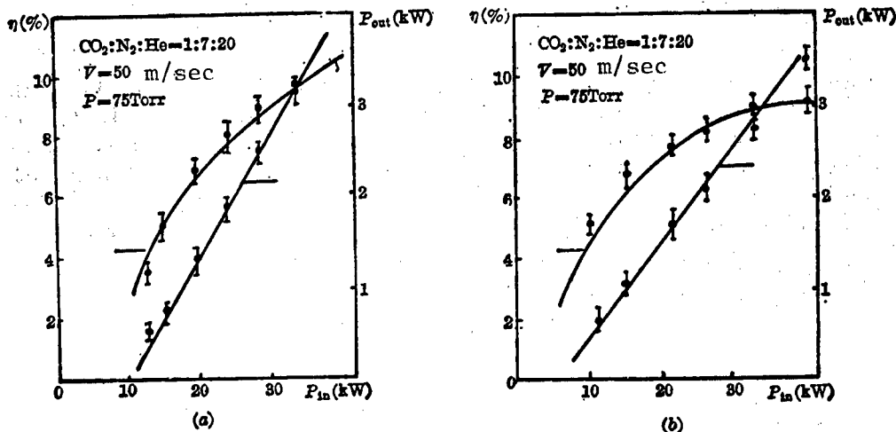
Figure 5. Theoretical (lines) and experimental (dots) output characteristics of the confocal unstable resonator
