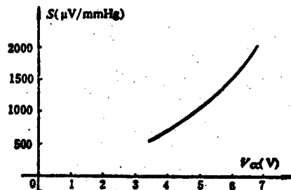
Figure 4. Relationship of sensitivity and voltage supplied
