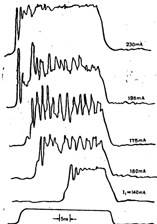
Figure 5. Transient Characteristics of 55 AlGaAs/GaAs CCTS DH Laser at I_2 = 215 mA
