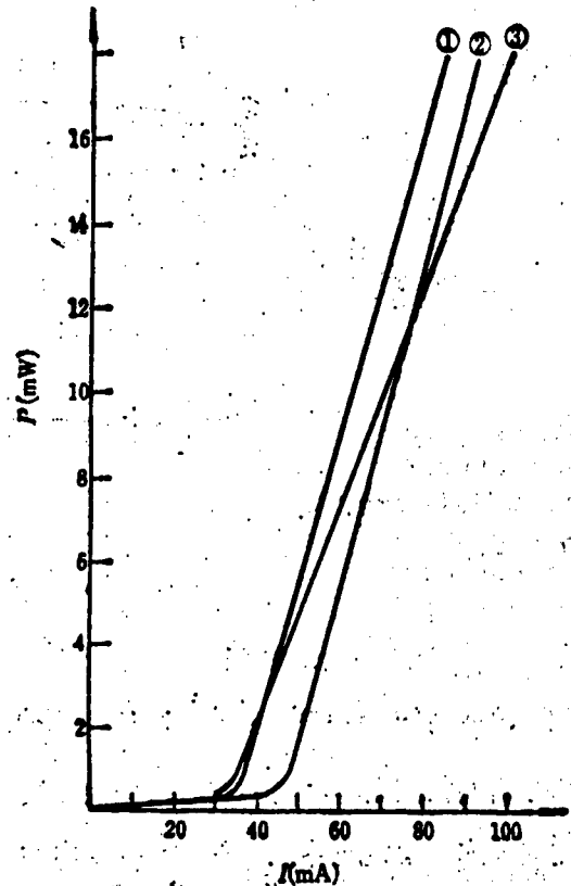
Figure 2. Light-power curves of SCP lasers: (1) SCP#037 (2) #040 (3) #039
