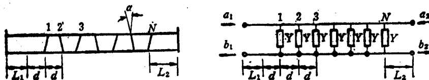
Figure 1 Waveguide H-Plan Slot Array and Its Equivalent Circuit
