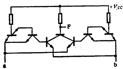
Figure 7. Exclusive-OR gate
