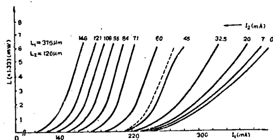
Figure 3. Light Intensity Versus Current L-I_2-I_1 Curves of 43 AlGaAs/GaAs CCTS DH Laser
