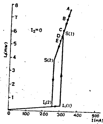
Figure 7. Bistable Characteristics of 83-A1 InGaAs/InP CCTS DH Laser Output
