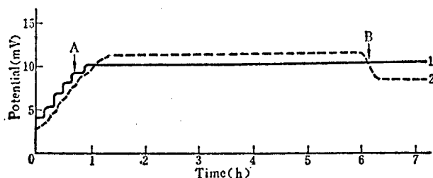
Fig.2 Curves obtained by XWT-264 recorder for input power and temperature at the bottom of the crucible respectively 1— mV value from pickup coil ( mV_P ), 2— mV value from silicon photocell ( mV_T )
