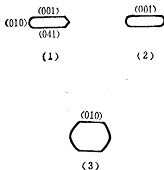
Fig.3 Cross section of alexandrite crystals
