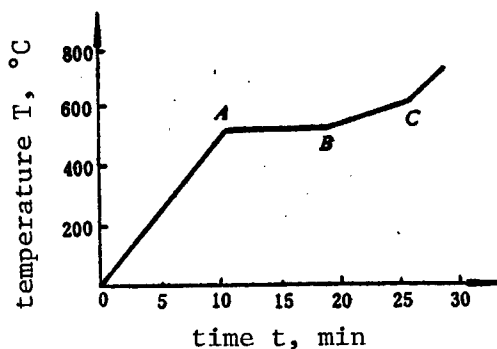
Figure 6. Sample Temperature Rising Curve
