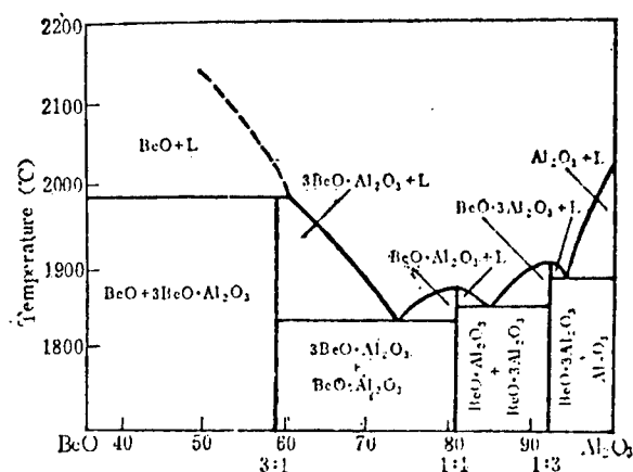
Fig.1 Phase diagram of BeO-Al 2 O 3 system after reference [10]
