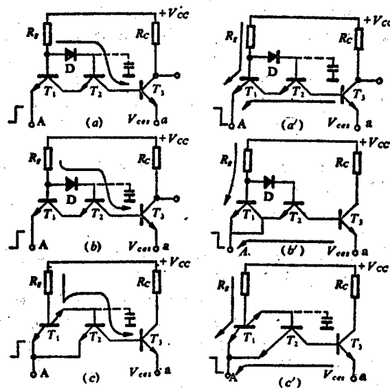
Figure 2. Structural forms of new simplified NAND gates
