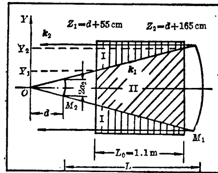
Figure 1. Divided regions and propagating waves in a positive-branch confocal unstable resonator
