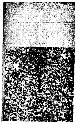
Figure 5. Aluminum-Graphite Containing 35 Percent Graphite X2
