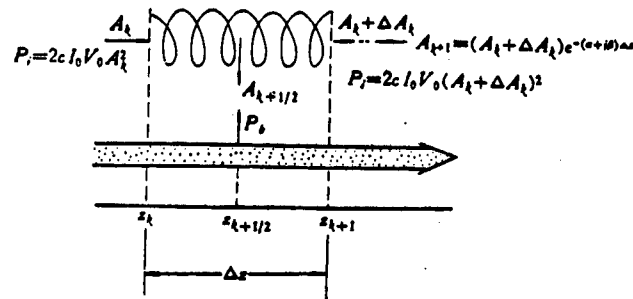
Figure 1. TWT Interaction Model (all A_k in the figure are \hat{A}_k )
