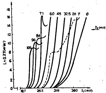
Figure 4. Light Intensity Versus Current L-I_2-I_1 Characteristics of the 22 AlGaAs/GaAs CCTS DH Laser
