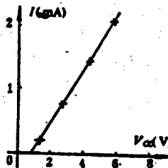
Figure 5. Relationship of power consumption current and supplied voltage
