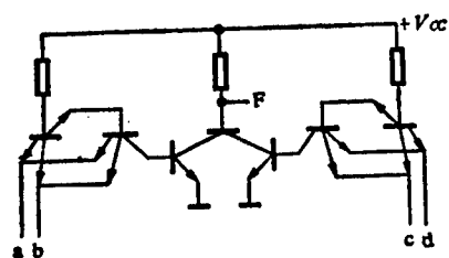
Figure 8. AND-OR-NOT gate
