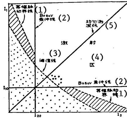
Figure 6. Pulsing Operation Region of CCTS DH Laser in the Phase Plane
