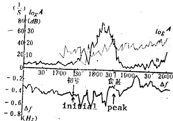
Figure 3. Variation of Amplitude Log A, Decay Rate n and Doppler Frequency Shift \Delta f of a High Frequency Signal Reflected by the Ionosphere With Time During the Solar Eclipse on 16 February 1980 in Yunnan
