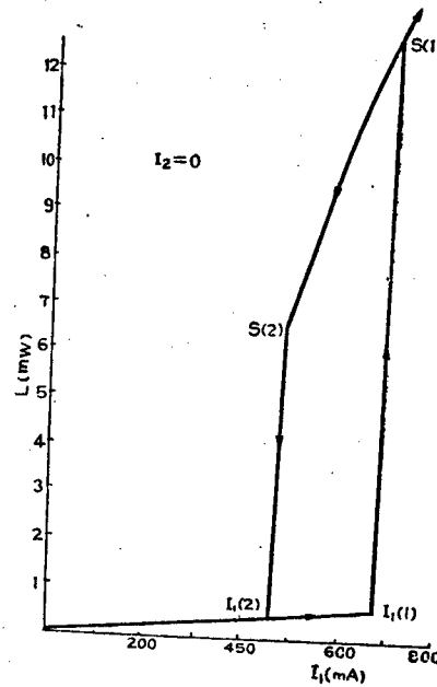
Figure 8. Bistable Characteristics of 83-815 InGaAs/InP CCTS DH Laser Output
