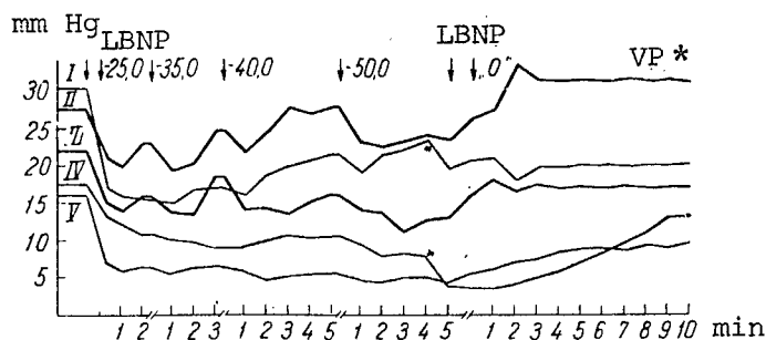
Figure 1. Dynamics of tissue pO_2 of gingival mucosa during LBNP (mm Hg) Vertical arrowheads show rarefaction in vacuum gear (mm Hg). The points on the curves show time of drastic worsening of wellbeing of subjects I and IV
