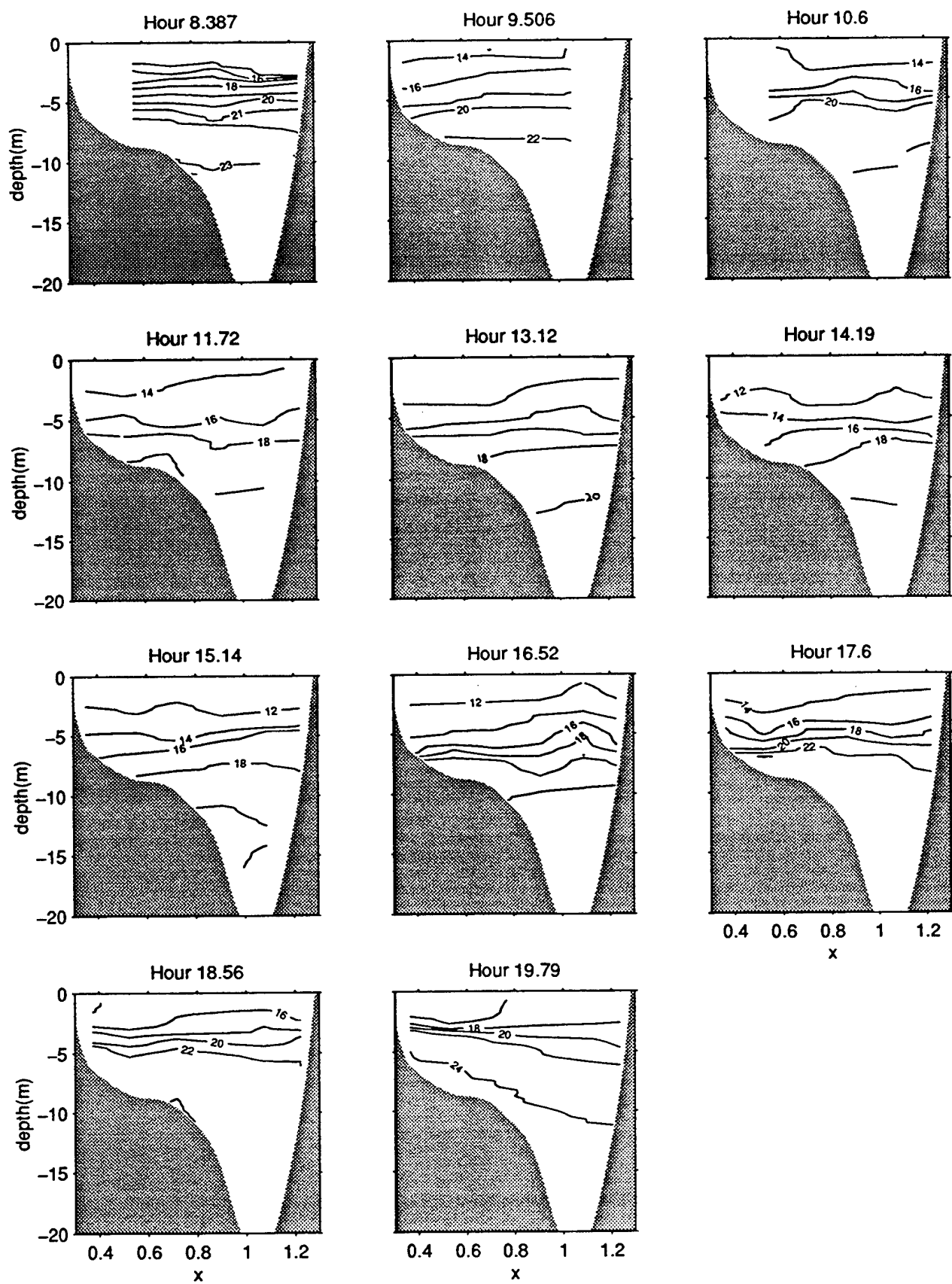
Figure 49a. North transect, salinity contours (psu) on 10/19/95
