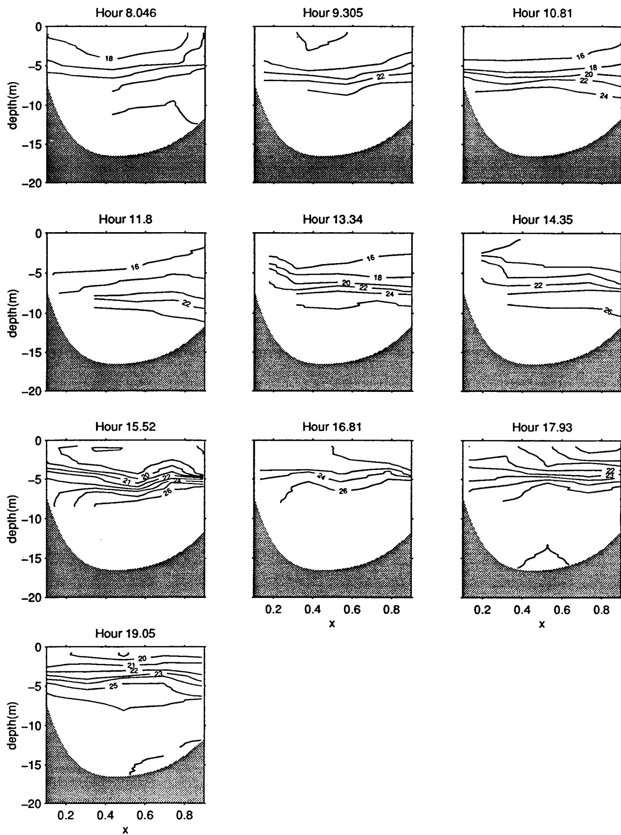
Figure 41a. South transect, salinity contours (psu) on 8/18/95
