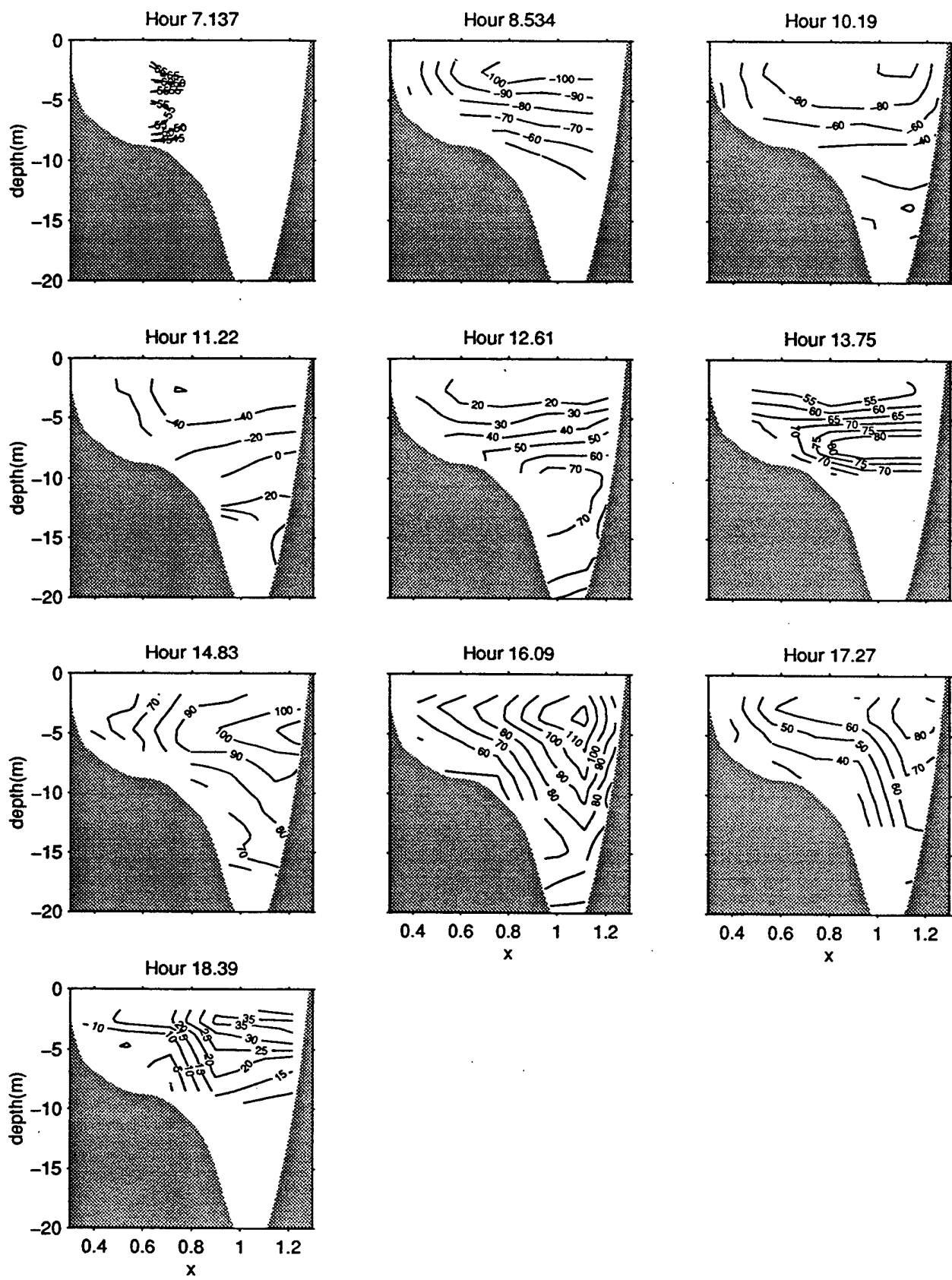
Figure 43b. North transect, velocity contours (cm/s) on 8/18/95
