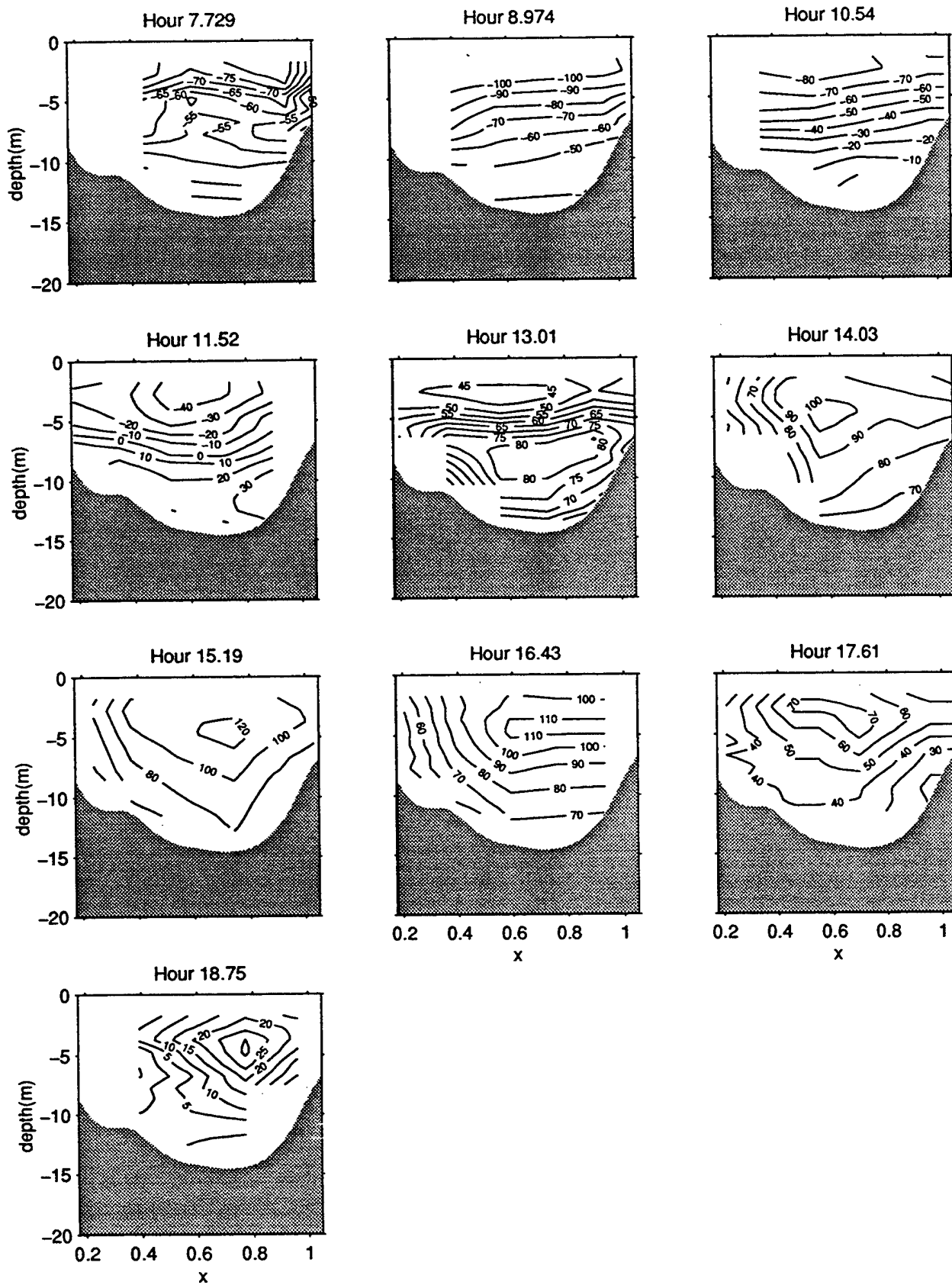
Figure 42b. Middle transect, velocity contours (cm/s) on 8/18/95
