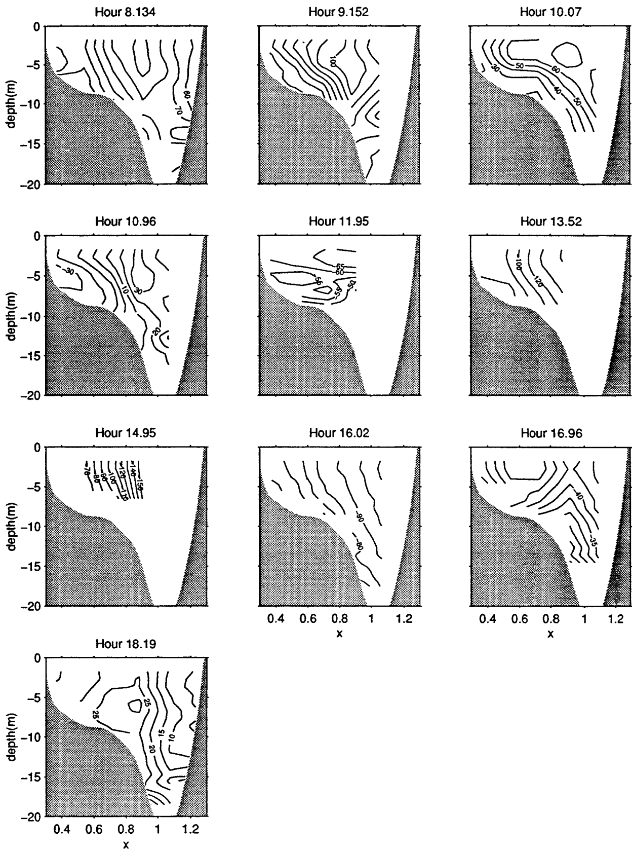
Figure 55b. North transect, velocity contours (cm/s) on 10/23/95
