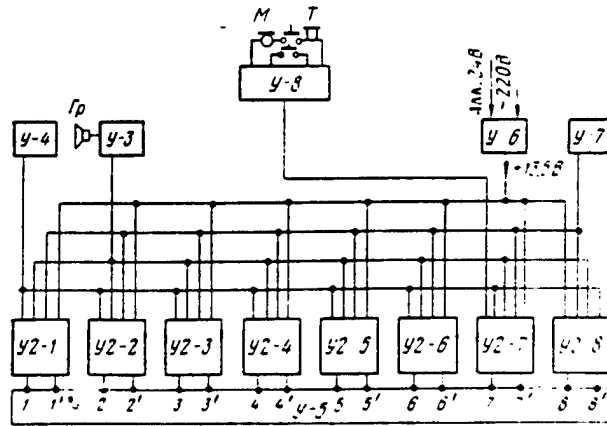
Sketch Block Diagram of PSS-6 Conference-Call Post
