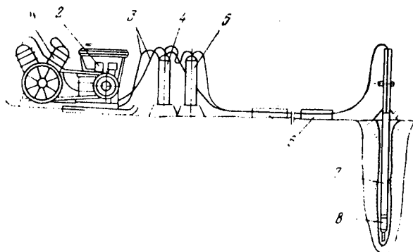
Figure 1. Basic Diagram of the MTBU-D Thermodrilling Unit
