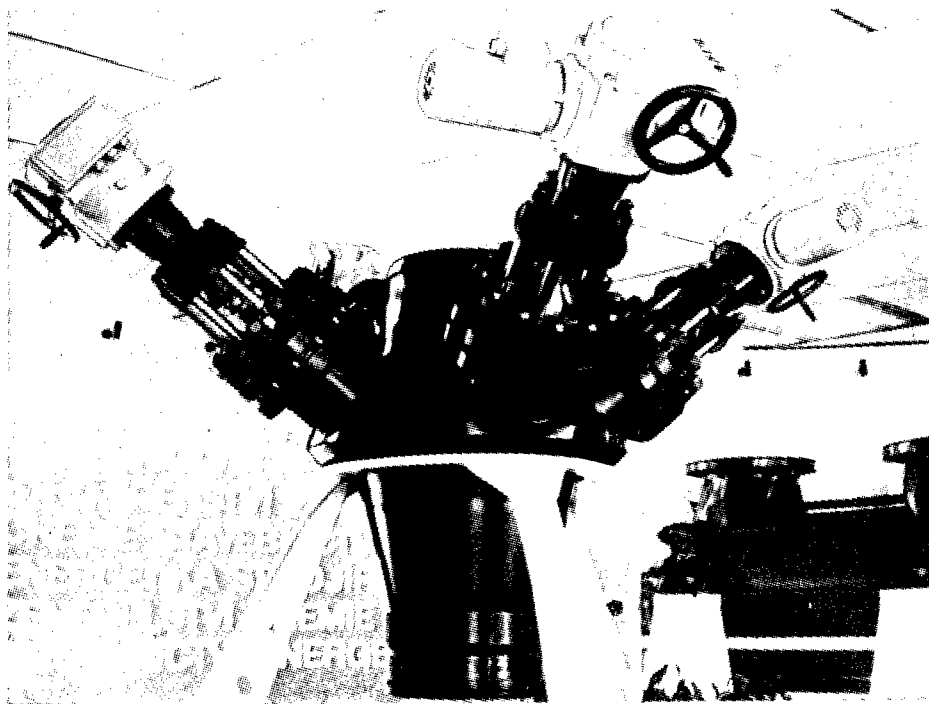
High-speed sector valve for AES's with fast-neutron reactors. Developed by the Sigma Scientific Research Institute [CSSR] and the Physical Energy Insititute in Obninsk [USSR]
