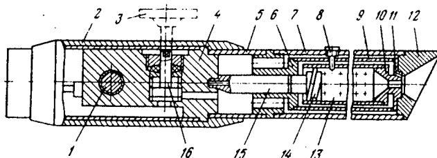
Figure 2. TBVD-60m Thermodrill
