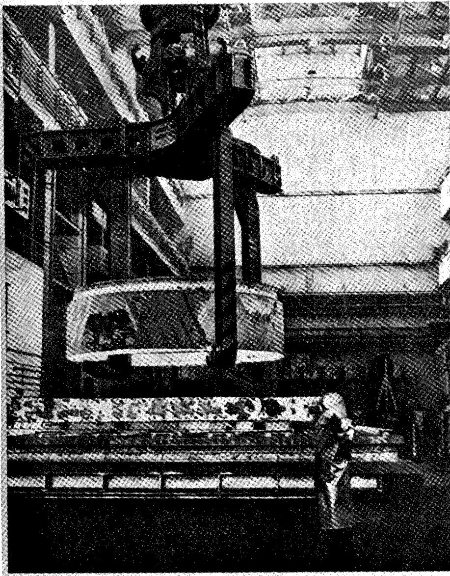
Billet for roof flange of VVER-1000 reactor
