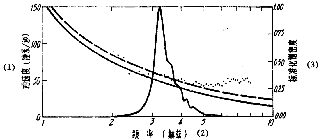
Figure 1. Relationship of Frequency and Phase Velocity of Wind-Wave Component at Low Wind Speed (Wind speed is 3 m/sec, water depth is 75 cm)
