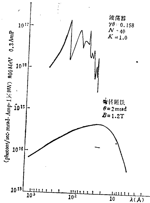
Figure 2. Radiation Spectrum of Undulator and Wanzhuan Magnet
