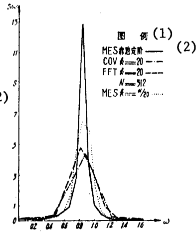
Figure 3. Spectrum Estimate (water pressure wave measurement record, N = 512 )
