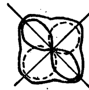
Figure 2. Directivity Chart
