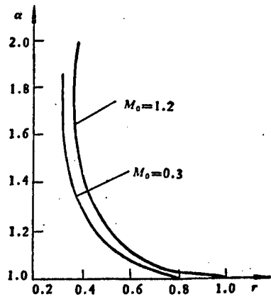
Fig. 4. Separation Coefficient Distribution D = -10, v_e = -10, \delta = -1.
