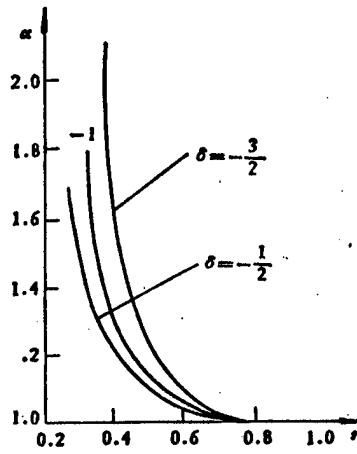
Fig. 3. Separation Coefficient Distribution D = -10, M_0 = 0.3, v_e = -10.
