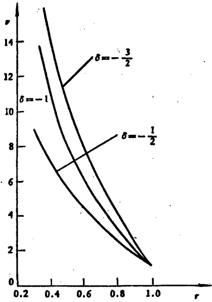
Fig. 2. Velocity Distribution D = -10, M_0 = 0.3, v_e = -10.
