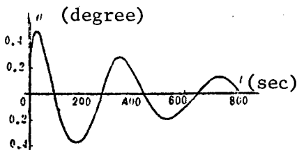
Figure 6. System Response Under Solar Radiation Torque
