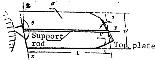
Figure 1. Schematic Diagram of the Spacecraft Structure
