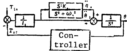
Figure 3. Transfer Function Block Diagram for Constrained Motion
