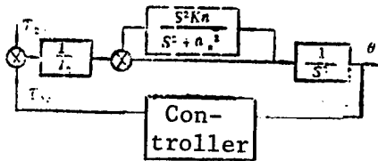
Figure 2. Transfer Function Block Diagram for Unconstrained Motion
