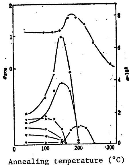
Figure 2. Annealing Behavior of Divacancy Band ( 2770\text{ cm}^{-1} ) and 6 New Absorption Bands
