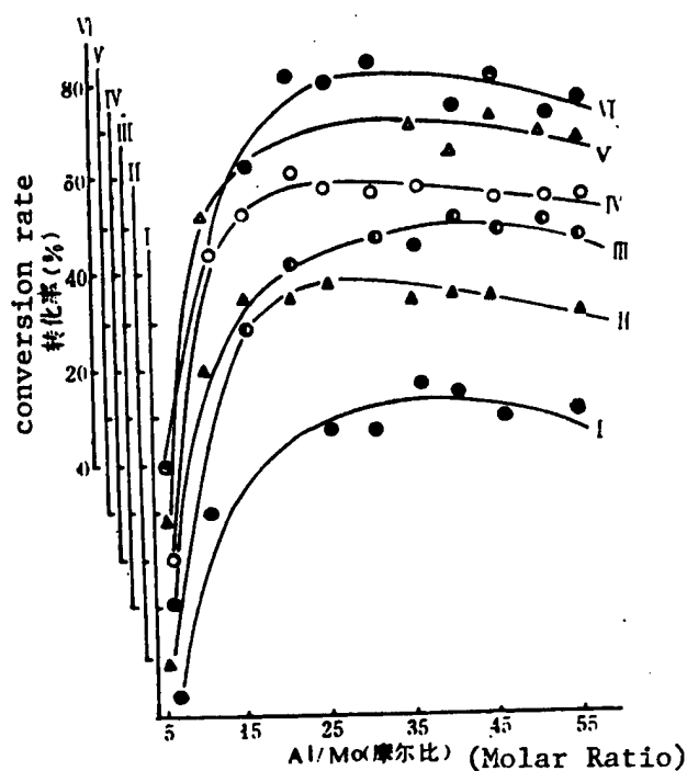
I. \text{MoCl}_4(\text{OC}_2\text{H}_5)_{4-n} ; II. \text{MoCl}_4(\text{OC}_3\text{H}_7)_{4-n} III. \text{MoCl}_4(\text{OC}_4\text{H}_9)_{4-n} ; IV. \text{MoCl}_4(\text{OC}_6\text{H}_{13})_{4-n} V. \text{MoCl}_4(\text{OC}_{10}\text{H}_{21})_{4-n} ; VI. \text{MoCl}_4(\text{OC}_{16}\text{H}_{33})_{4-n} \text{ROH}/\text{Mo} = 8 ; \text{Mo}/\text{Bd} = 2.0 \times 10^{-4} ; 50^\circ\text{C} ; 7小时 hours
