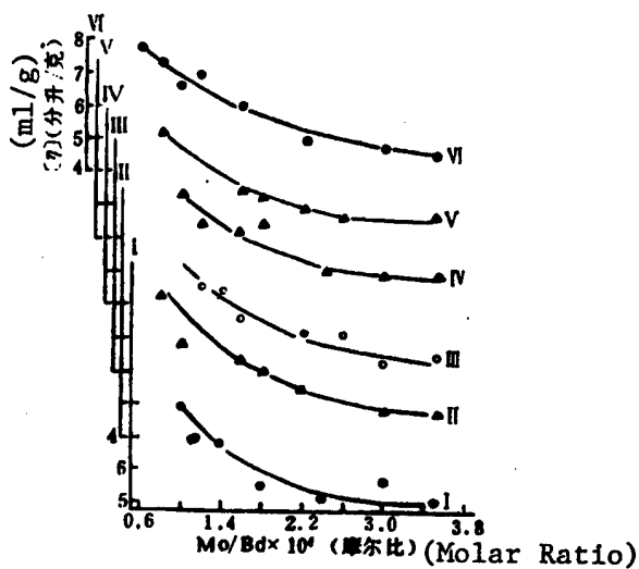
Figure 6. Effect of Mo Dosage on Inherent Viscosity
