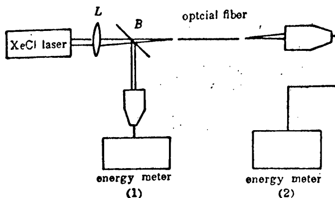
Figure 1. Schematic of the experimental setup for measuring the XeCl laser transmission characteristics through an optical fiber
