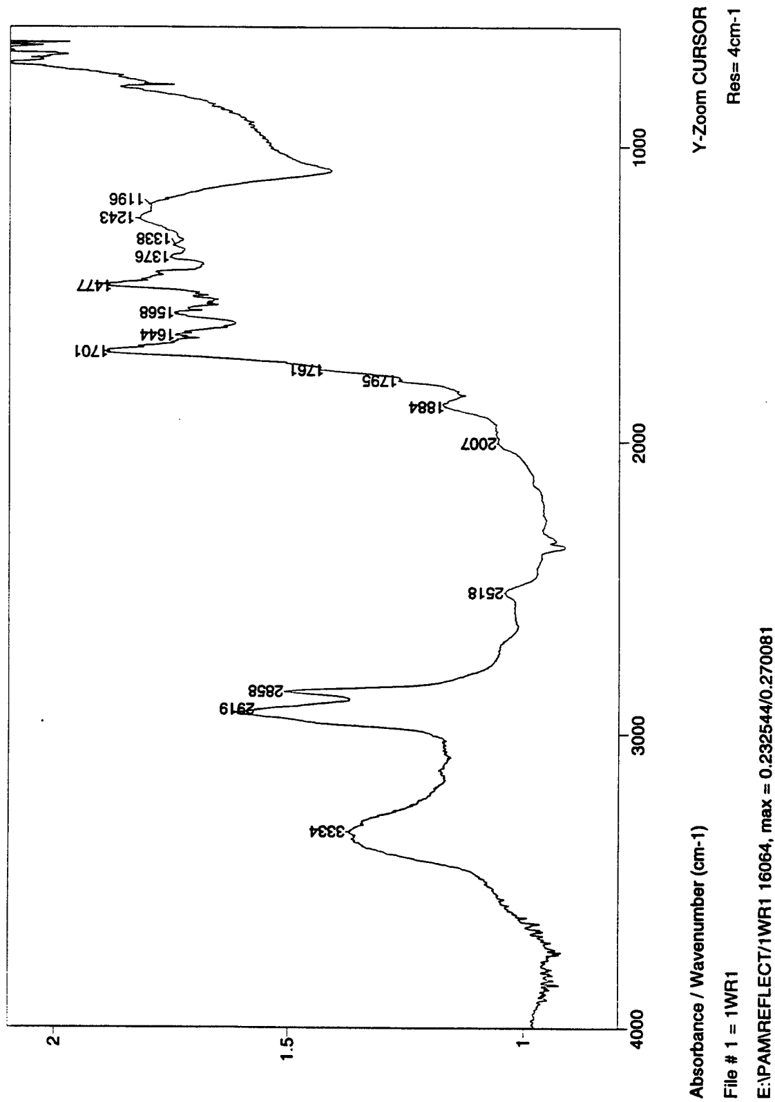
Figure 19. Reflectance IR Spectrum of the Plasma-Treated One-Pack Green Paint.
