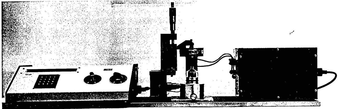
Fig. 3. Induction heater set-up for fibre embedment into PEEK.
