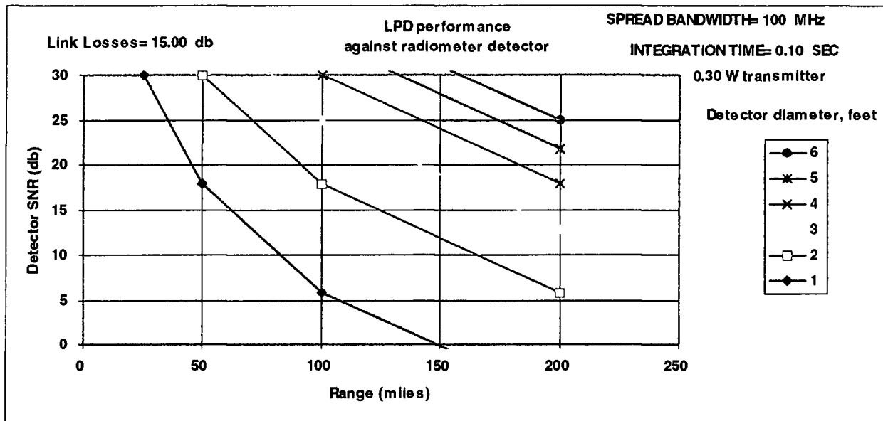
Figure V-9 Radiometer Signal-to-Noise Ratio for a Simple Scenario
