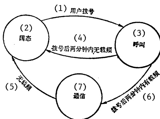
Figure 5. Diagram of Telephone Line State Change
