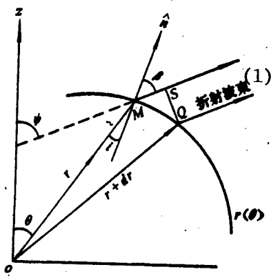
Figure 3. Geometry of Surface of Revolution Array Lens
