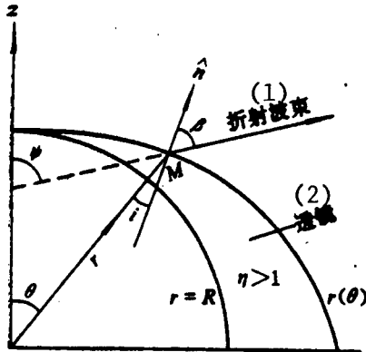
Figure 5. Dielectric Lens
