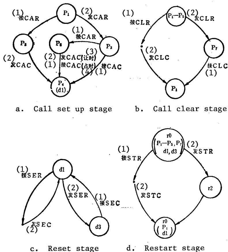
Figure 2.2. Logic Channel State Diagram
