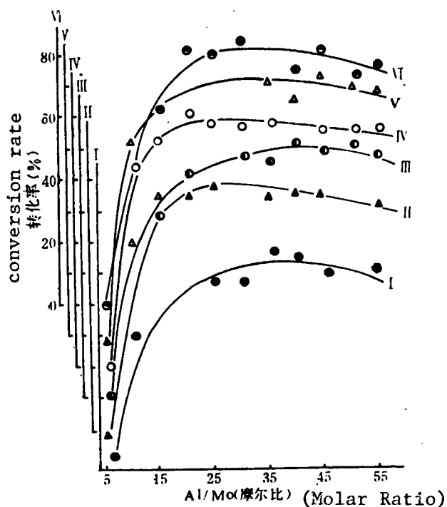
I. \text{MoCl}_n(\text{OC}_2\text{H}_5)_{4-n} ; II. \text{MoCl}_n(\text{OC}_3\text{H}_7)_{4-n} III. \text{MoCl}_n(\text{OC}_4\text{H}_9)_{4-n} ; IV. \text{MoCl}_n(\text{OC}_6\text{H}_{13})_{4-n} V. \text{MoCl}_n(\text{OC}_{10}\text{H}_{21})_{4-n} ; VI. \text{MoCl}_n(\text{OC}_{16}\text{H}_{33})_{4-n} \text{ROH}/\text{Mo} = 8 ; \text{Mo}/\text{Bd} = 2.0 \times 10^{-4} ; 50^\circ\text{C} ; 7小时 hours
