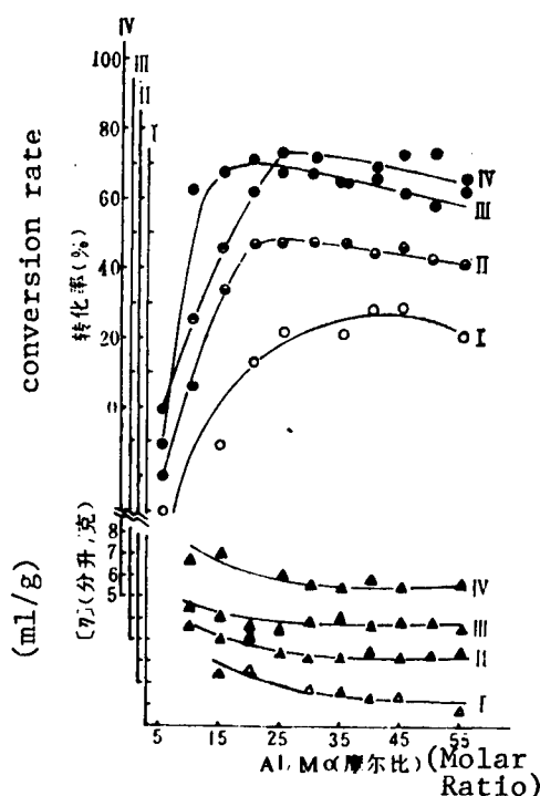
I. \text{MoCl}_n(t\text{-OC}_4\text{H}_9)_{4-n} ; II. \text{MoCl}_n(\text{S-OC}_4\text{H}_9)_{4-n} ; III. \text{MoCl}_n(i\text{-OC}_4\text{H}_9)_{4-n} ; IV. \text{MoCl}_n(i\text{-OC}_2\text{H}_5)_{4-n}
