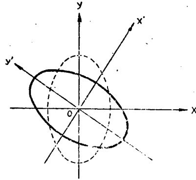
Figure 3. Fixed Coordinate System and a Rotating Coordinate System in Twisted Optic Fiber
