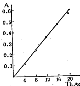
Fig. 8 Calibration Curve
