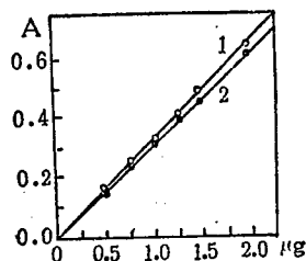
Figure 2. Calibration Curve
