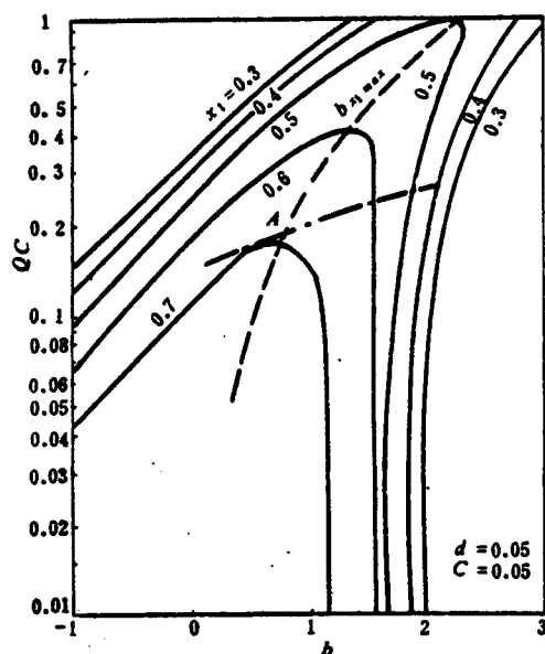
Figure 1. Parameters obtained from Kats's relational equation
