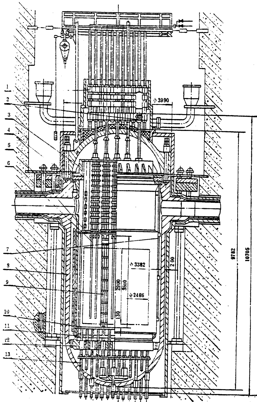
Figure 2. The Reactor
