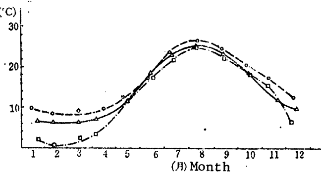
Figure 5: Annual changes in surface layer temperature at the three test sites
