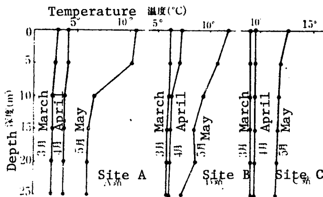
Figure 4: Temperature changes with depth at 3 measurement sites
