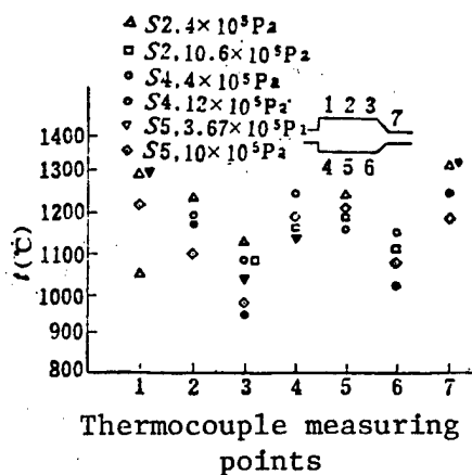
Figure 5. Wall Temperature
