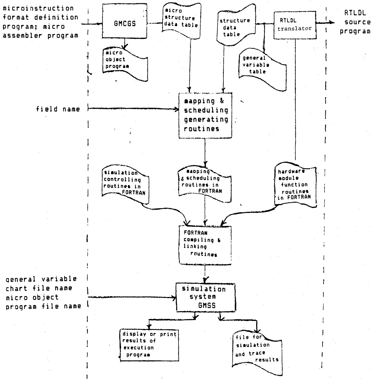
Figure 1. Flowchart for CADSMDS System Structure
