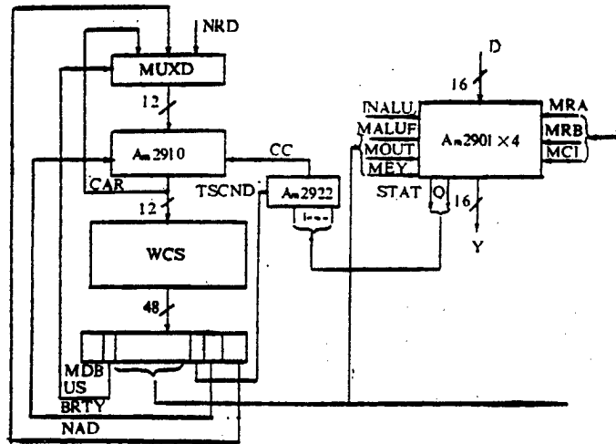
Figure 5. CPU Block Diagram of a Model Computer
