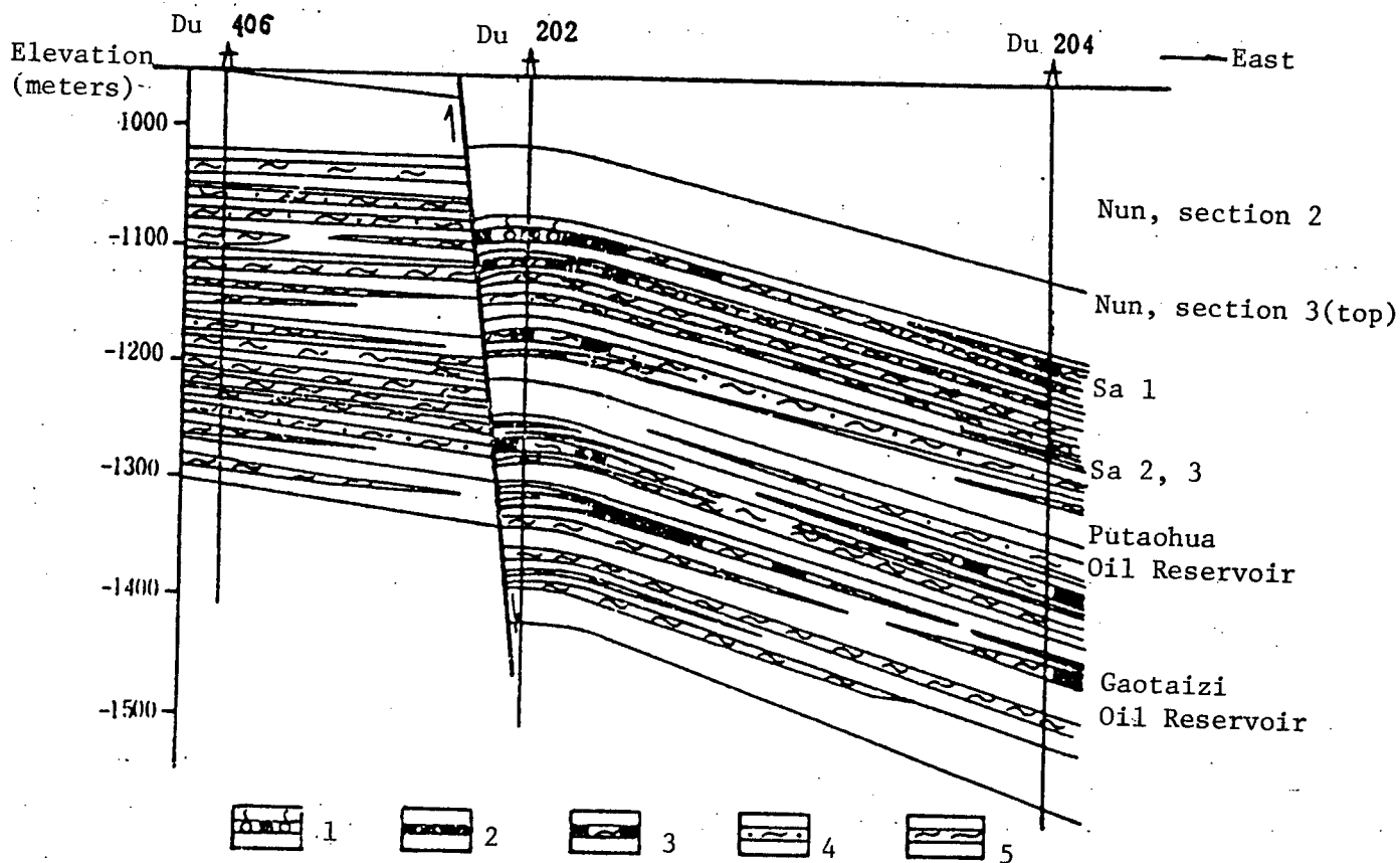
Figure 5. Cross-section of Xindian Oil Pools
