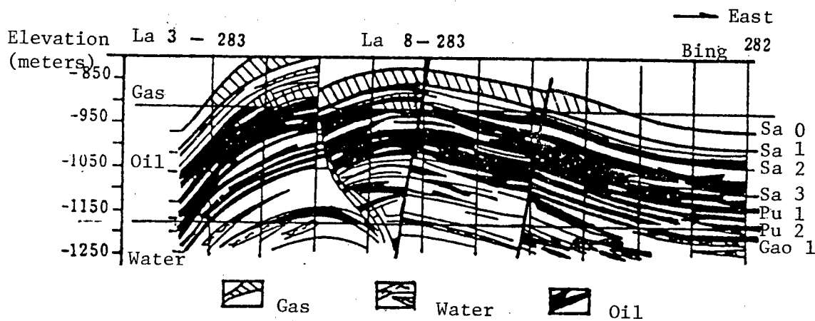
Figure 2. Cross-section of Lamadian Oil and Gas Pools
