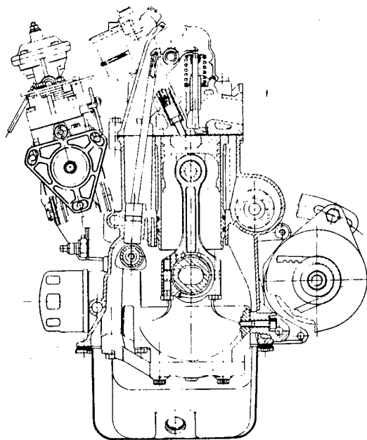
Fig 7 - Section view of 2-cylinder engine.
