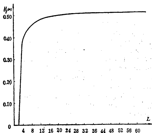
Figure 1. Relationship Between H_f(\mu) and the Gray Level Scale L
