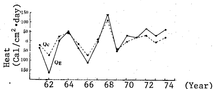
Figure 3. The Weighted Average and Yearly Variation Curves of the Latent and Sensible Heat of the Kuroshio Region in February
