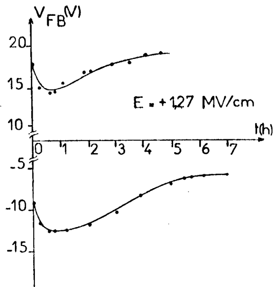
Figure 13. Shift of the C(V) curve under the effect of a field of 1.27 \times 10^6 \text{ V/cm} and 80 percent of relative humidity.
