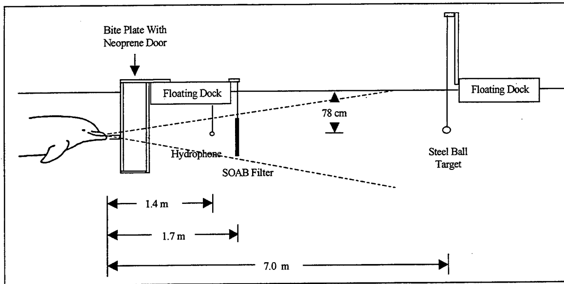
Figure 4.12 Echolocation Experiment Showing Dolphin's Projected Sonar Beam
