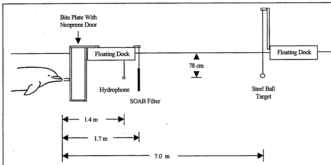
Figure 4.1 Echolocation Experiment Configuration
