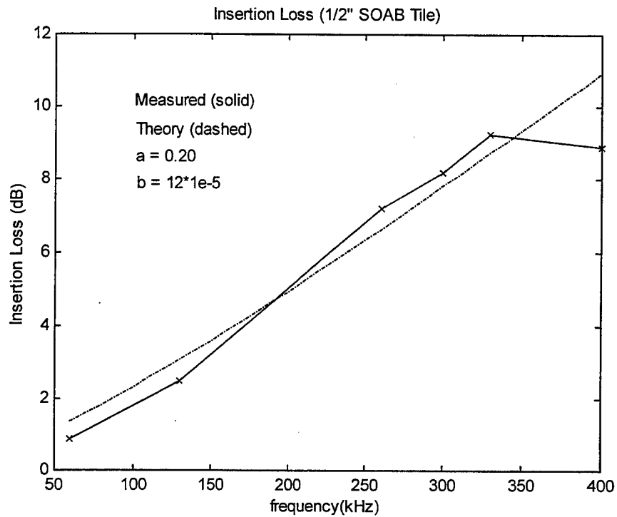
Figure 3.7 Experimental And Theory Insertion Loss
