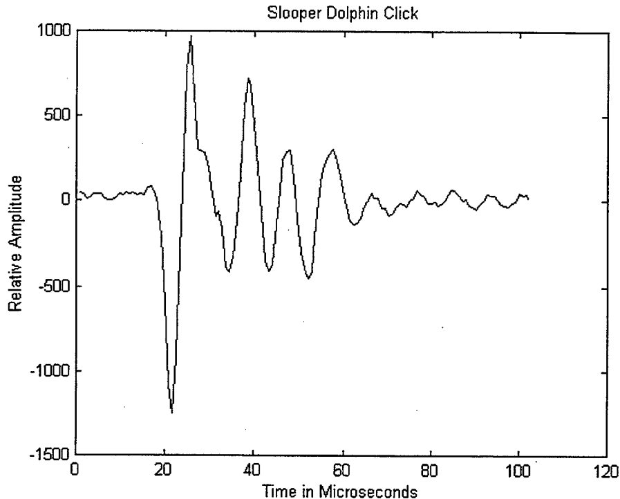
Figure 2.7 Bottlenose Dolphin Echolocation Click
