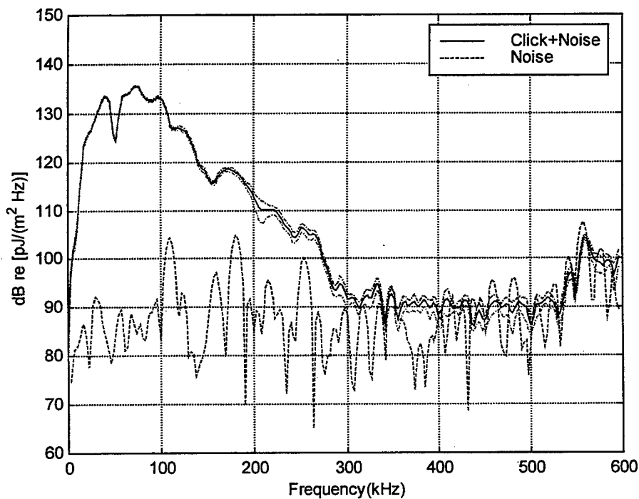
Figure 4.8 Eight Dolphin Clicks And Corresponding Average Energy Flux Spectral Density With No Filter Present ( \pm 1\sigma shown as dot-dash line)
