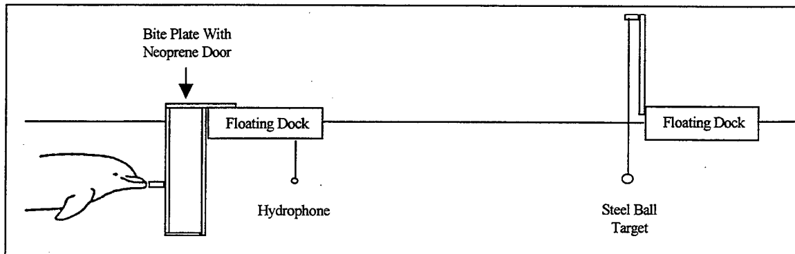
Figure 2.5 Generic Experimental Geometry
