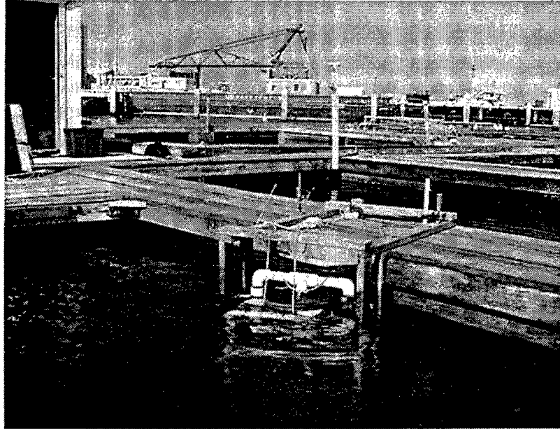
Figure 4.5 Photo of Experiment Configuration Showing Bite Plate and Target Stand
