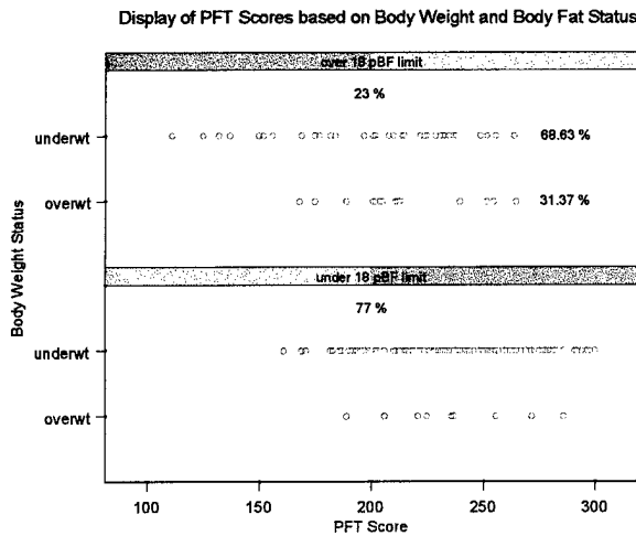
Figure 4. Relationship of Body Weight and Body-Fat Status's with PFT Score. The upper panel indicates that 68.63% of Marines deemed fat are actually under their maximum weight limits. The lowest PFT scores are associated with this group of Marines (data set 1).
