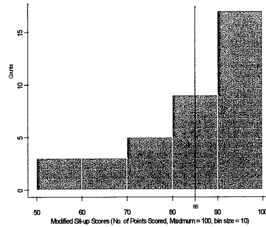
Figure 12. Histogram of Sit-Up Scores and Modified Sit-Up Scores. Current Sit-Up Mean = 76.13 for 92.5 points (data set 1). Modified Sit-Up Mean = 85.46 for 85 points (data set 4).
