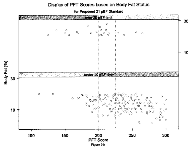
Figure 9. Comparison of the Relationships between the 18 and 20 percent B.F. Limits with Respect to PFT Scores. Comparing the top panels for 9 (a), and 9 (b) indicates that there are less first class PFT qualifying scores for the group of Marines deemed over 20 percent B.F., than there are in the group deemed over 18 percent B.F. (data set 1).
