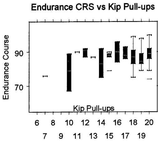
Figure 3. 2 Boxplots Comparing Trends in Mean Pull-Up Scores Based on other Events (Data Set 3).
