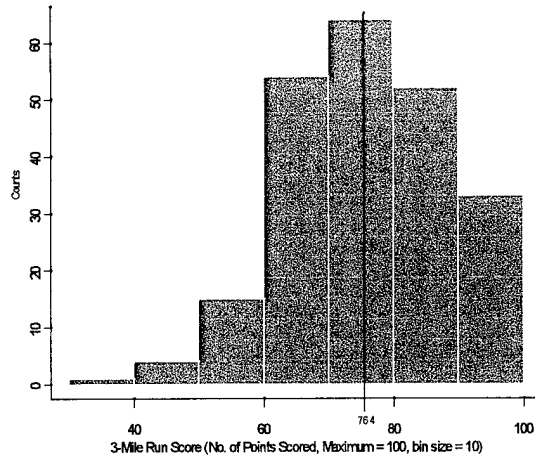
Figure 11. Histogram of Pull-Up Scores (data set 1). The Average Pull-Up Score = 60 points out of 100 points possible, which equates to the Median of 12 pull-ups performed, with the Mean = 12.85. Histogram of 3 Mile Run Scores (data set 1). Mean = 21.86 minutes for 76.4 points.
