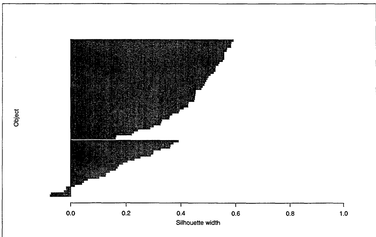
Figure 4.3 Silhouette Plot of Function "pam".
