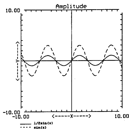
Figure 3: Amplitude The dotted wave is the same wave from Figure 1. The wave represented by the solid line is only half as loud as the first wave. The second wave would sound much softer than the first wave.
