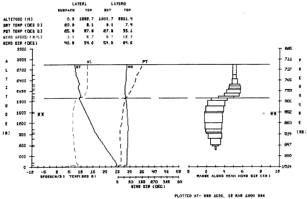
Figure 1: Meteorological Output Plot from REEDM Version 7.08 for B-33 Mission Using T-0.8h Rawinsonde Data.
