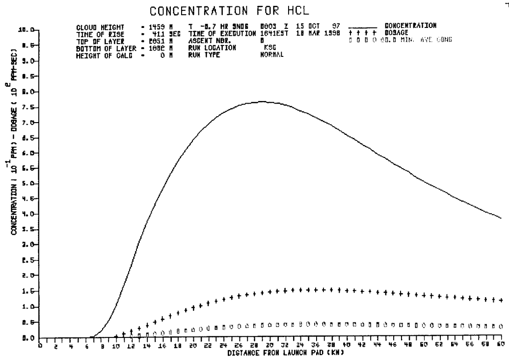
Figure 4: Meteorological Output Plot from REEDM Version 7.08 for B-33 Mission Using T-0.8h Rawinsonde Data.
