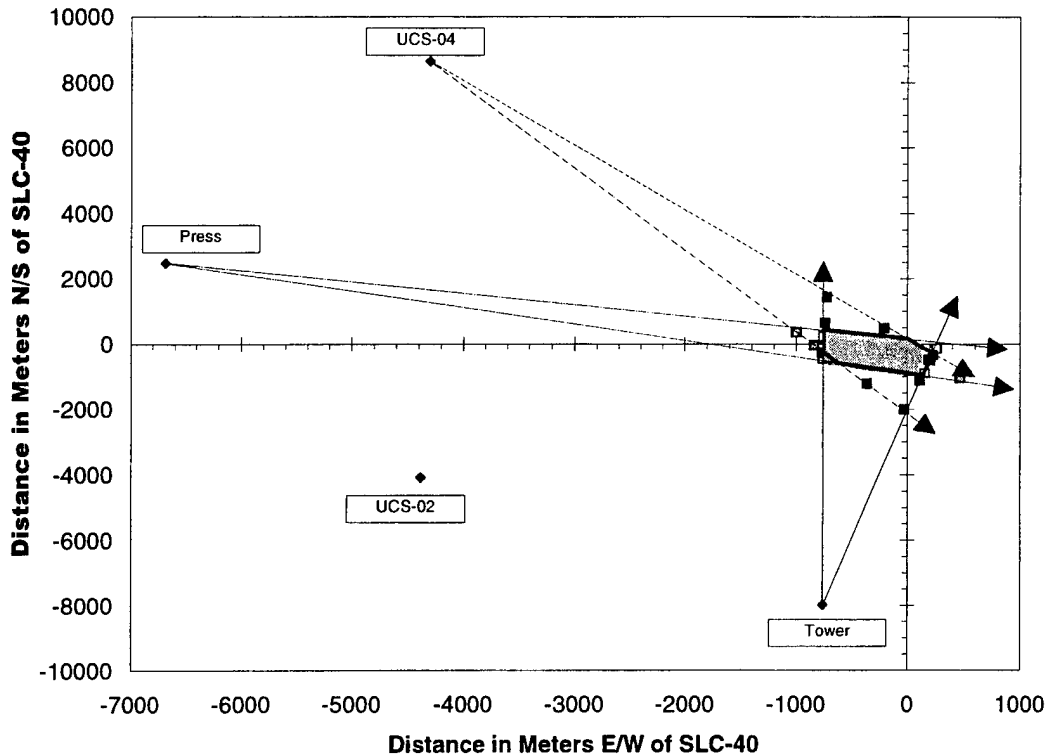
Figure 2. Comparison of the #B33 cloud extent derived from the PLMTRACK polygon analysis and from the PLMVOL analysis (i.e., shaded area within PLMTRACK polygon). The imager positions and rays are actual #B33 data for T+01:30 (mm:ss) after launch.
