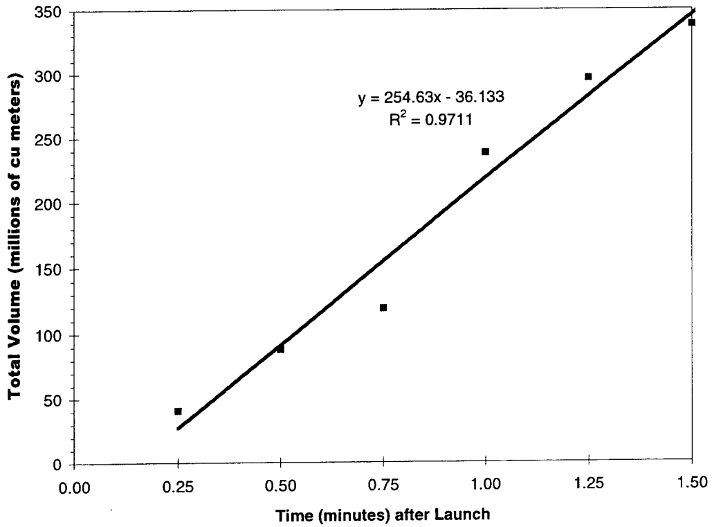
Figure 16. Cloud volume versus time.
