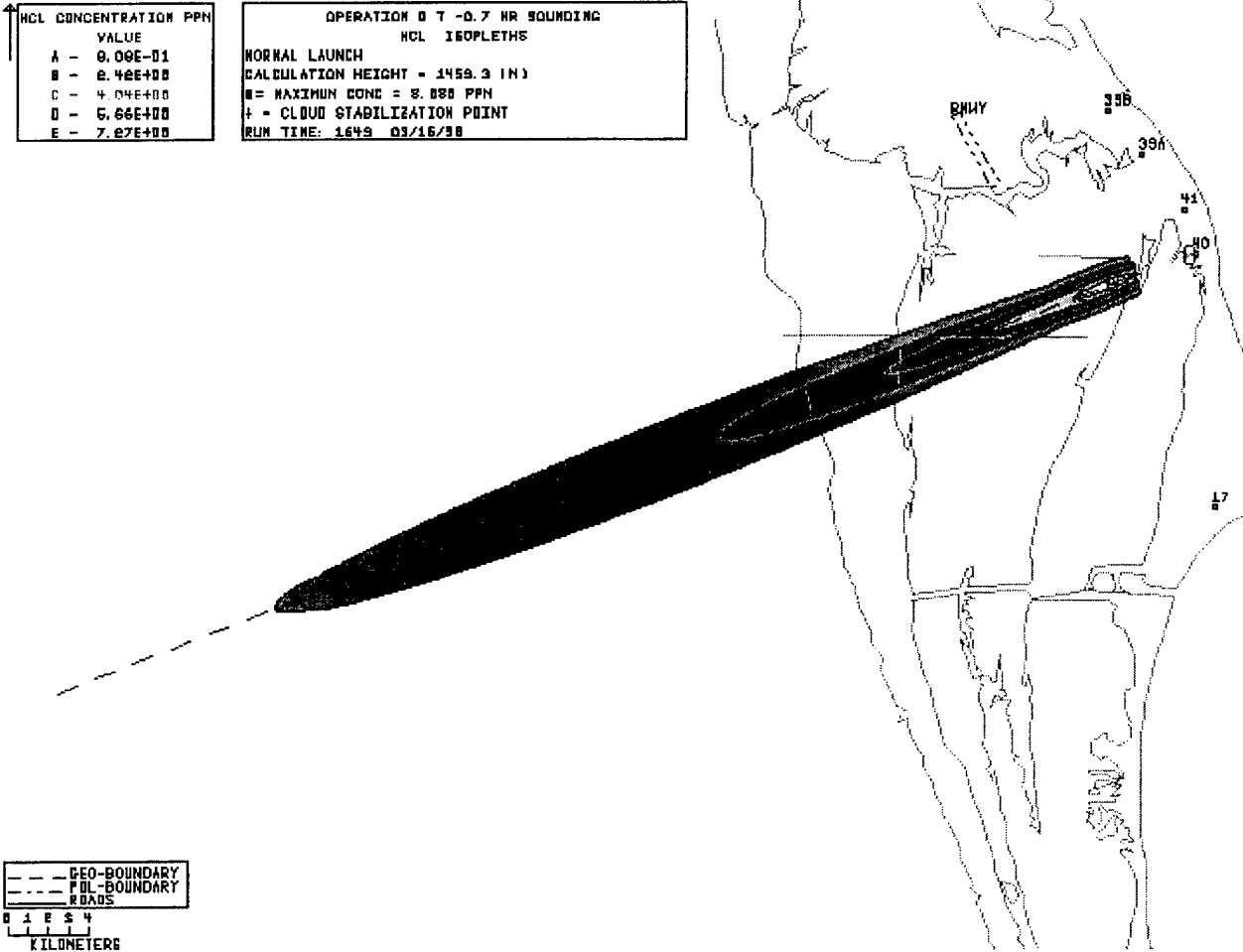
Figure 3: HCl Stabilization Height Concentration Isopleth Predictions from REEDM Version 7.08 for B-33 Mission Using T-0.8h Rawinsonde Data.
